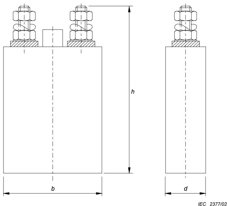
Figure 1 – Example of a sealed prismatic cell with two terminals
