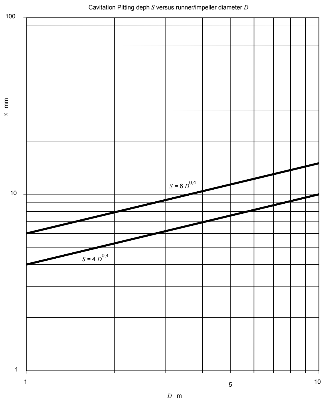
Figure A.1 – Examples of maximum permissible values of cavitation-pitting depth for runners/impellers
