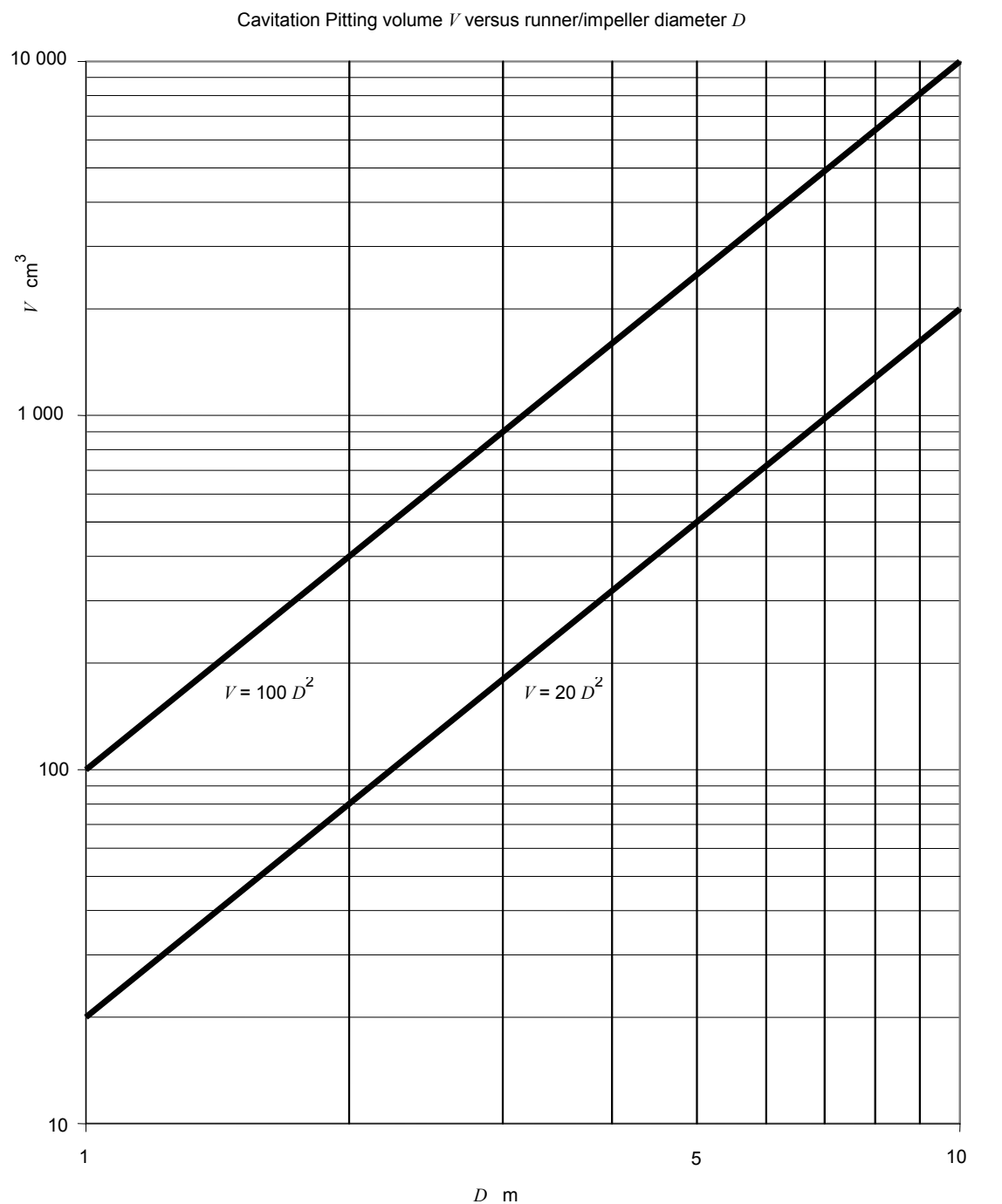
Figure A.2 – Examples of maximum permissible values of cavitation-pitting volume for runners/impellers
