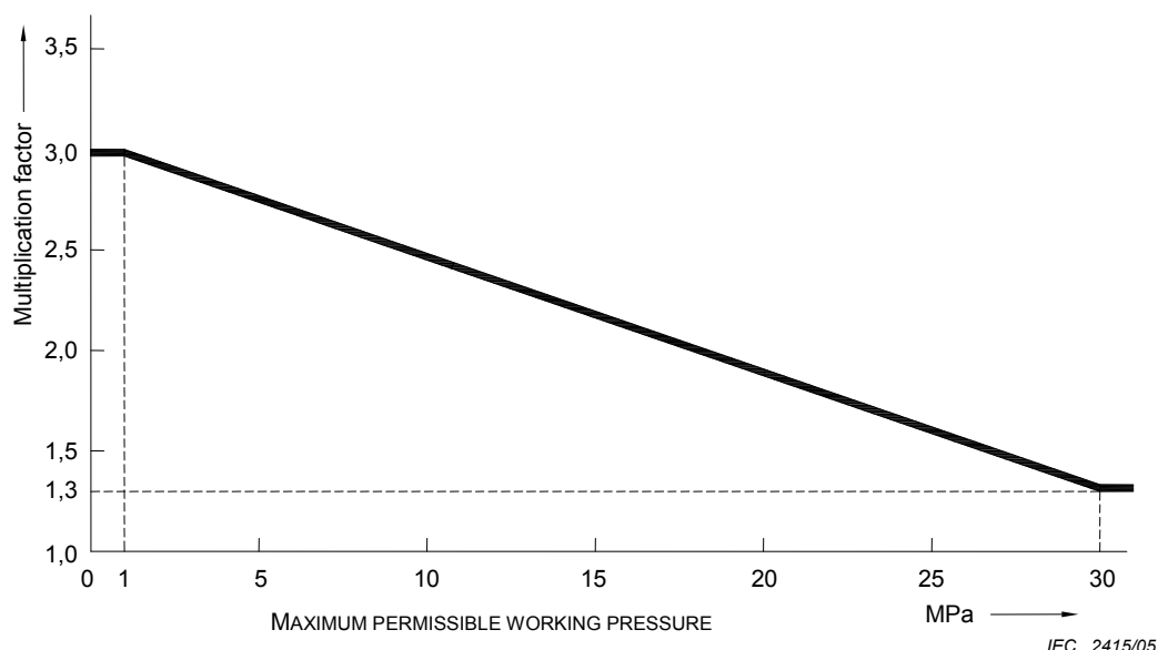
Figure 32 – Ratio between HYDRAULIC TEST PRESSURE and MAXIMUM PERMISSIBLE WORKING PRESSURE (see 9.7.5)
