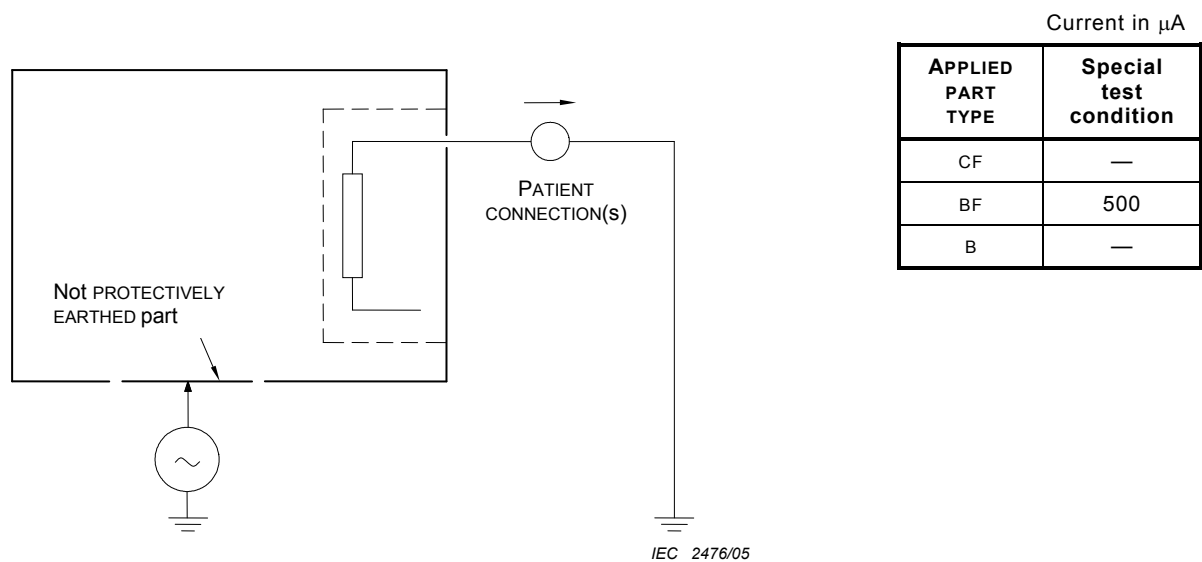
Example with the measuring supply circuit of Figure F.1. Figure K.5 – ME EQUIPMENT with a PATIENT CONNECTION of a TYPE BF APPLIED PART that is not PROTECTIVELY EARTHED (simplified Figure 18) (see 8.7.4.7 d))
