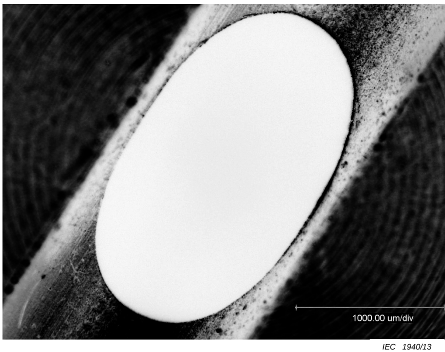
Figure 9 – Example of different quality achievements of the surface finish of the fan jet nozzle
