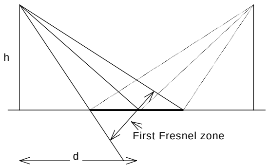
Figure A.6d – Width of absorber
