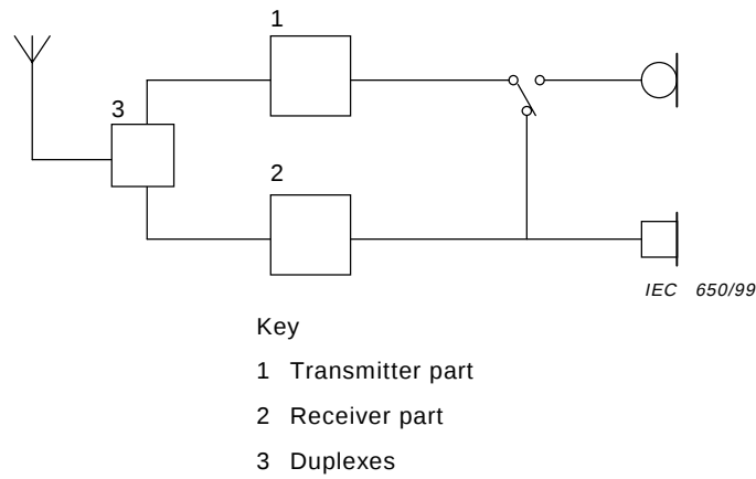
Figure A.20a – Loop-back arrangement for analogue modulation equipment
