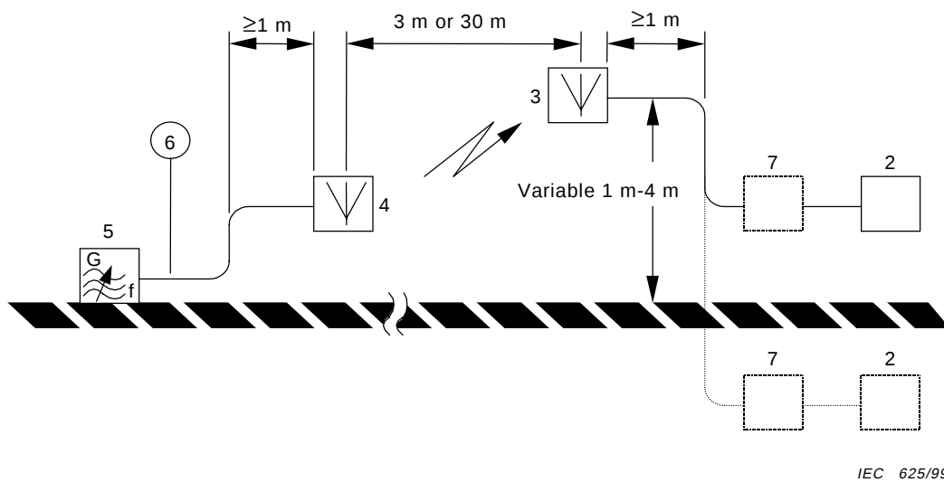
Figure A.1b – Measuring arrangement for substitution measurement
