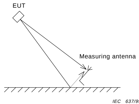
Figure A.7 – Higher position to reduce ground-reflected wave
