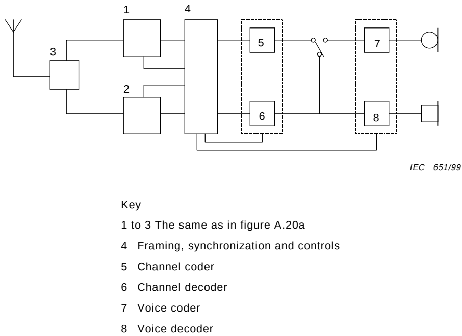
Figure A.20b – Loop-back arrangement for digital modulation equipment
