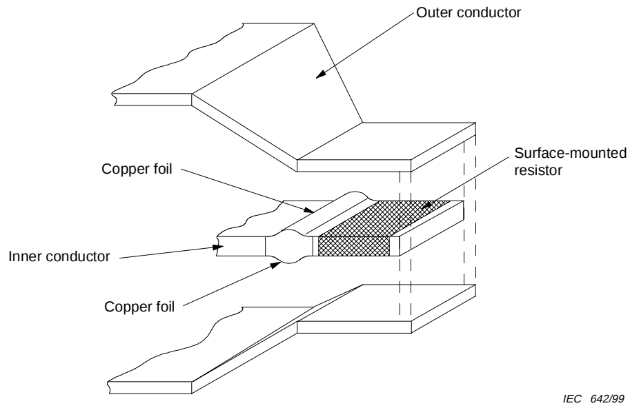
Figure A.12 – Detail of stripline load
