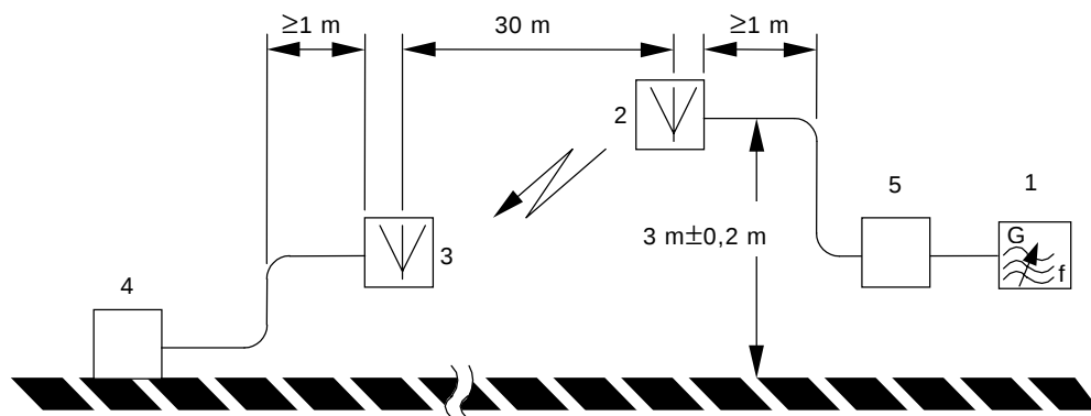
Figure A.2a – Measuring arrangement for calibration measurement
