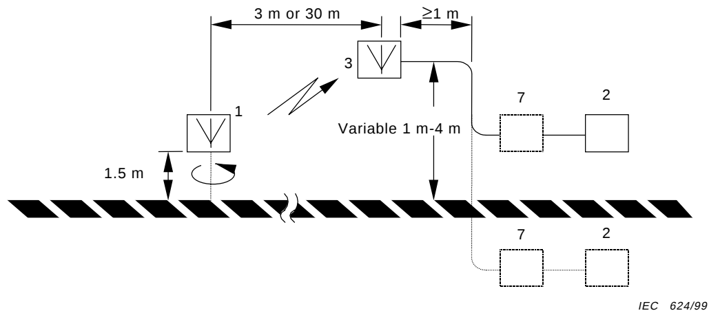
Figure A.1a – Measuring arrangement for the EUT
