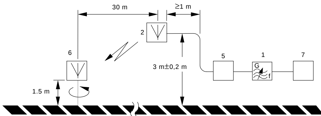
Figure A.2b – Measuring arrangement for the EUT
