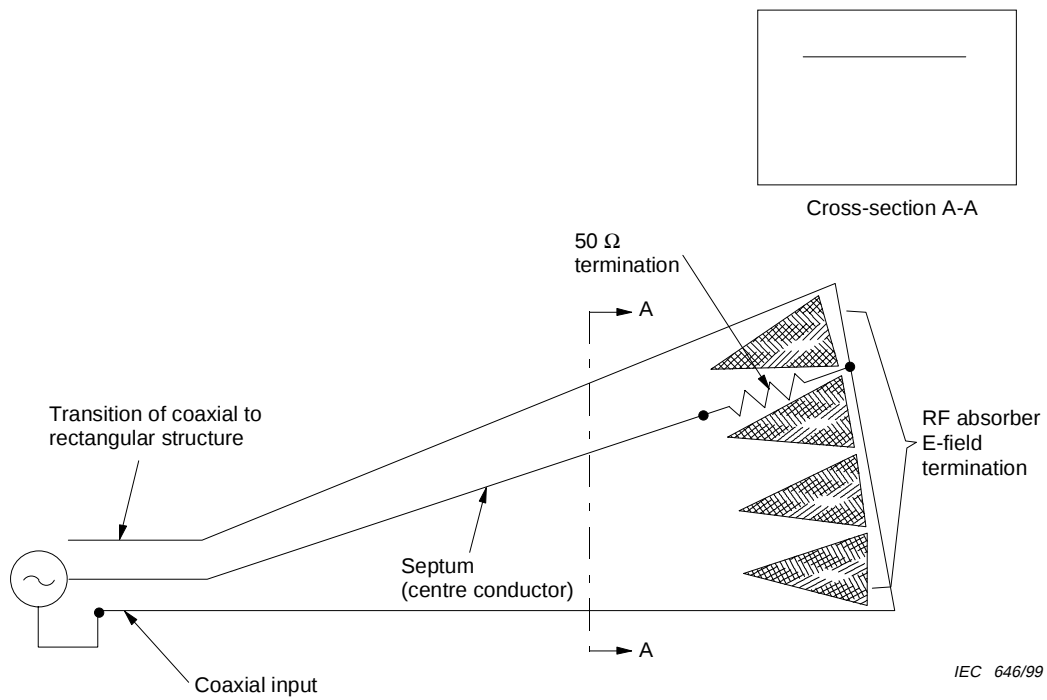
Figure A.16 – Example of a GTEM cell construction
