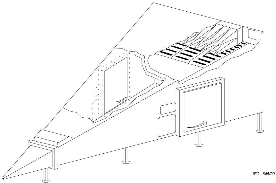
Figure A.15 – Example of a GTEM cell
