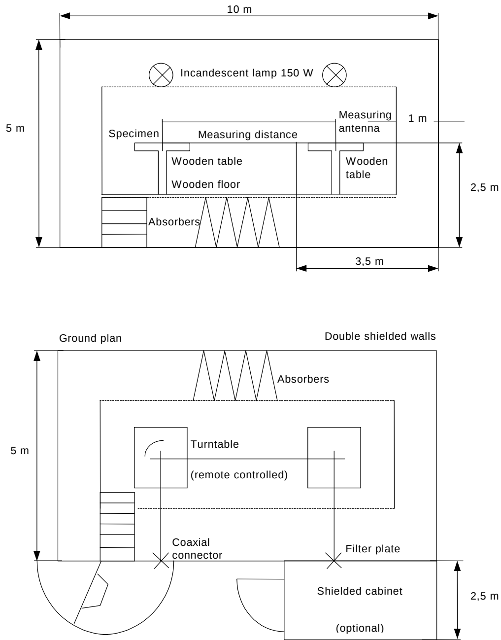
Figure A.8 – Example of an anechoic chamber
