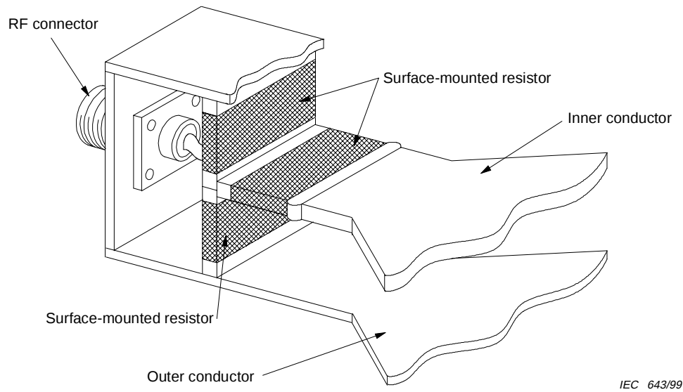
Figure A.12 – Detail of stripline load
