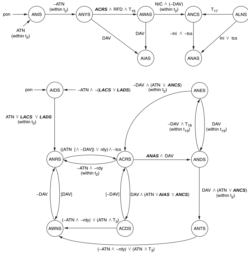
Figure 6—AH state diagram
