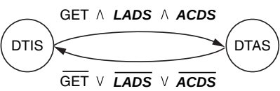
Figure 15—DT state diagram
