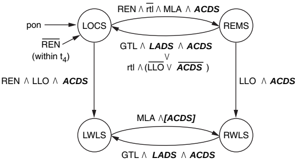
Figure 12—RL state diagram
