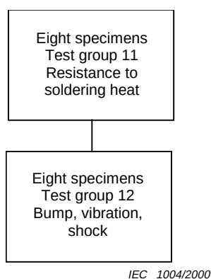
Figure 9 – Test plan for mounting CQCs
