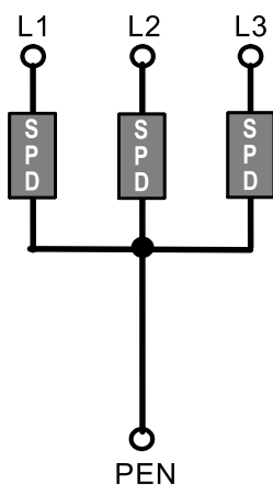
Figure 534.3 – Connection type CT1 (3+0-configuration) for a three-phase system
