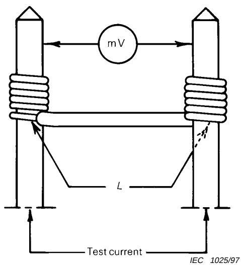
Figure 8a – Conventional wrapped connections
