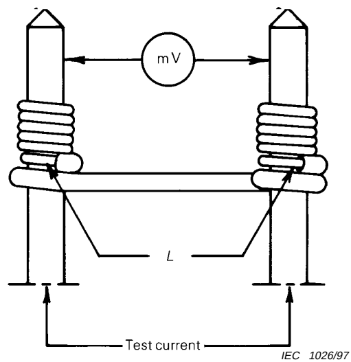
Figure 8b – Modified wrapped connections
