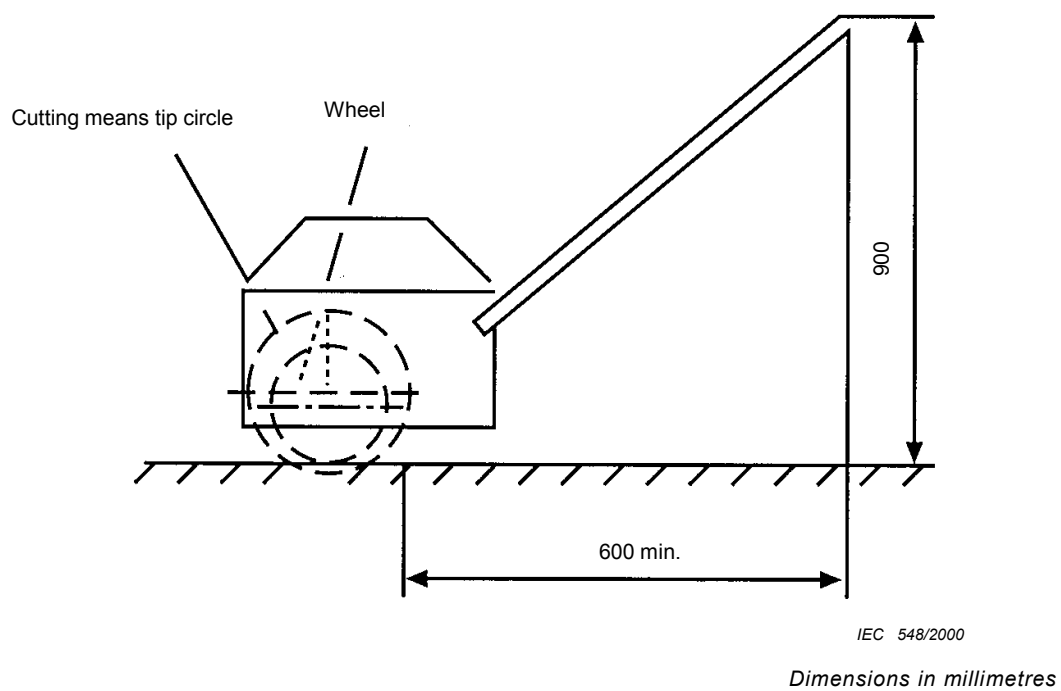
Figure 102 – Safety distances – Other lawn scarifiers and aerators
