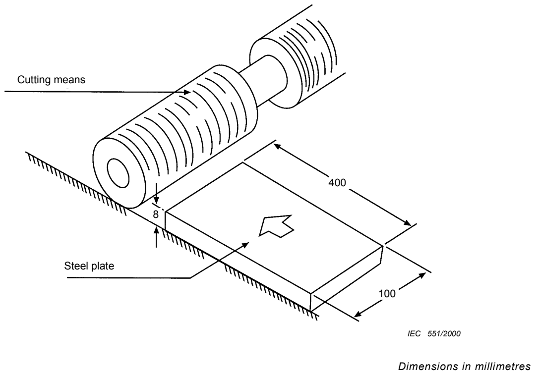
Figure 105 – Strength of cutting means
