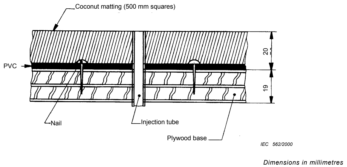
Figure BB.1 – Thrown object test fixture base detail
