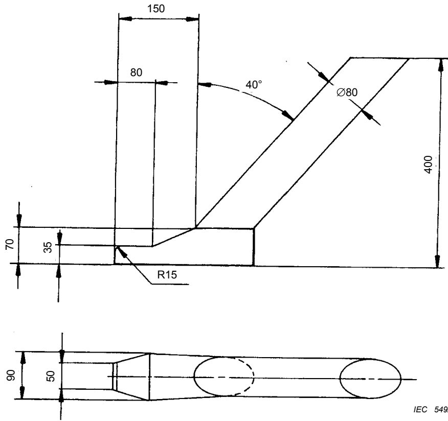
Figure 103 – Foot probe
