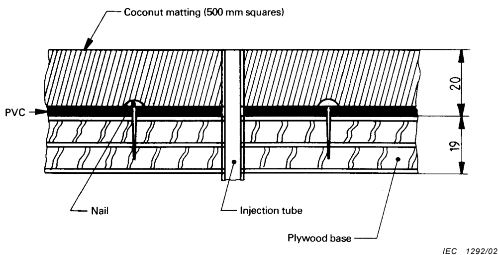
Figure CC.1 – Thrown object test fixture – Base detail
