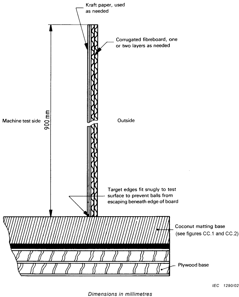
Figure BB.4 – Test enclosure walls and base
