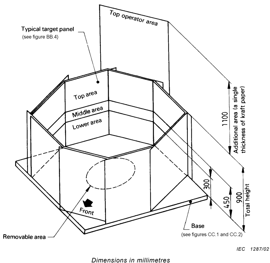
Figure BB.1 – Thrown object test fixtures – General layout
