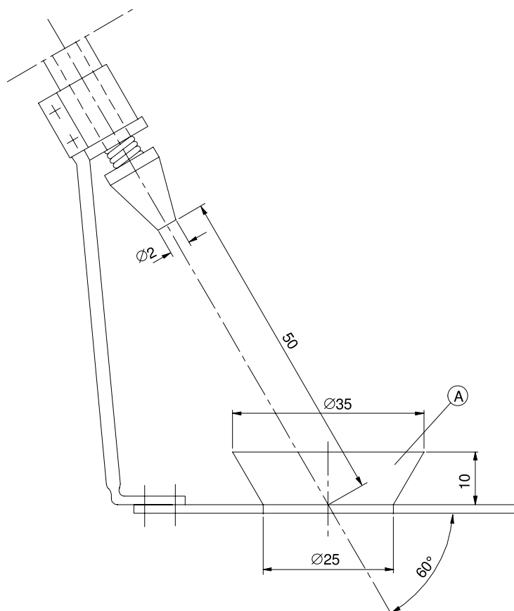
Figure 102 – Probe for measuring surface temperatures
