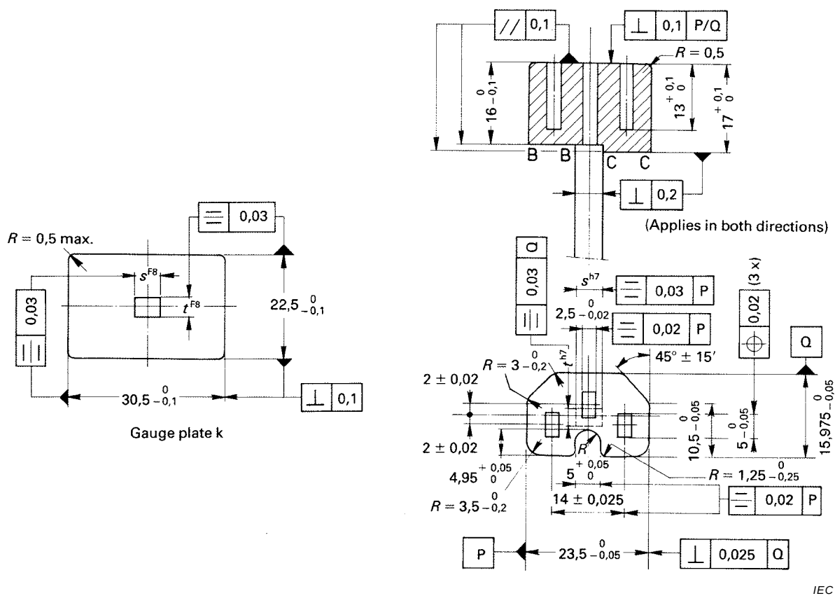
Figure 16 – "GO" gauge for appliance inlets to standard sheets C14, C16 and C18
