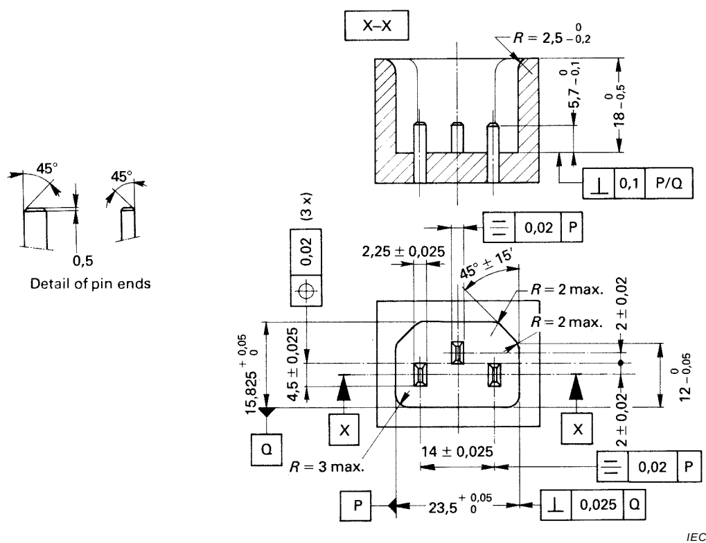
Figure 14 – "GO" gauge for connectors to standard sheet C13
