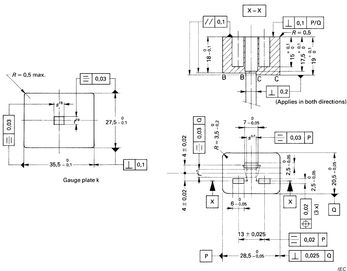
Figure 20 – "GO" gauge for appliance inlets to standard sheets C20 and C24
