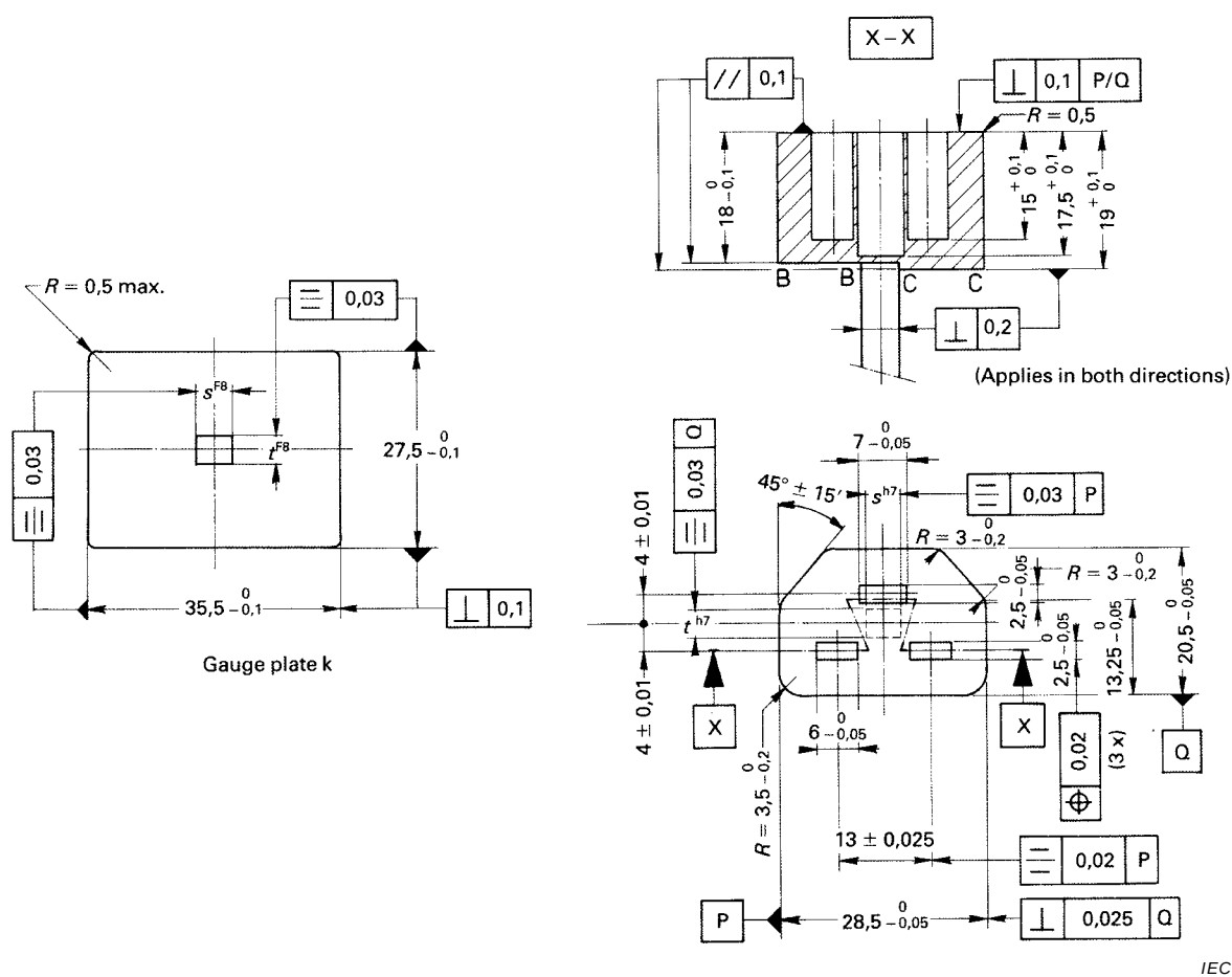
Figure 22 – "GO" gauge for appliance inlets to standard sheet C22
