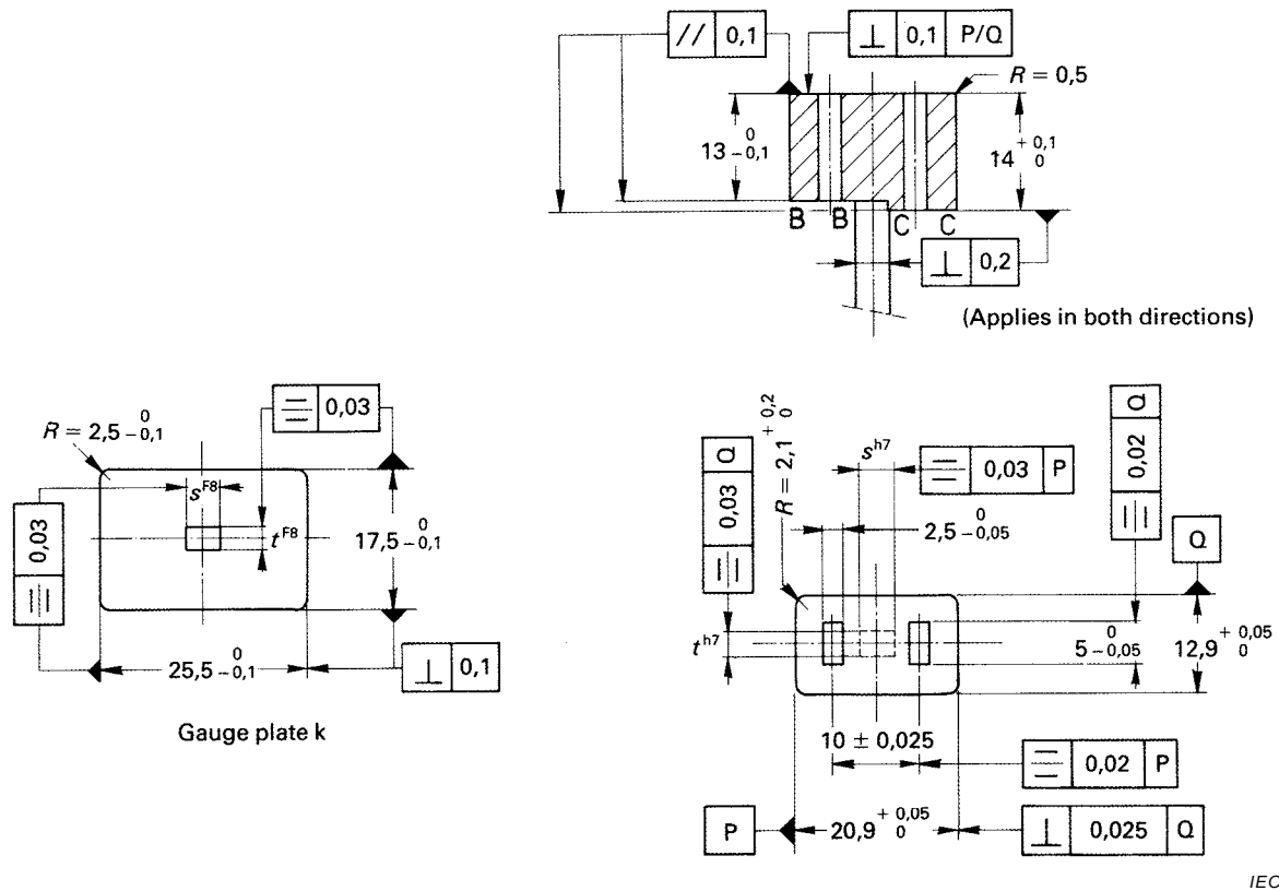
Figure 13 – "GO" gauge for appliance inlets to standard sheets C10
