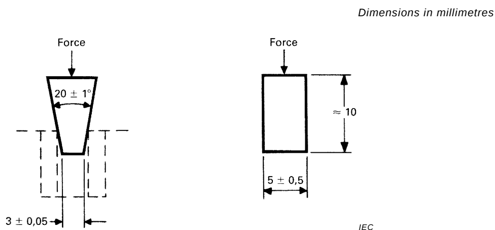
Figure 10 – "NOT-GO" gauge for appliance inlets to standard sheets C8, C8A and C8B
