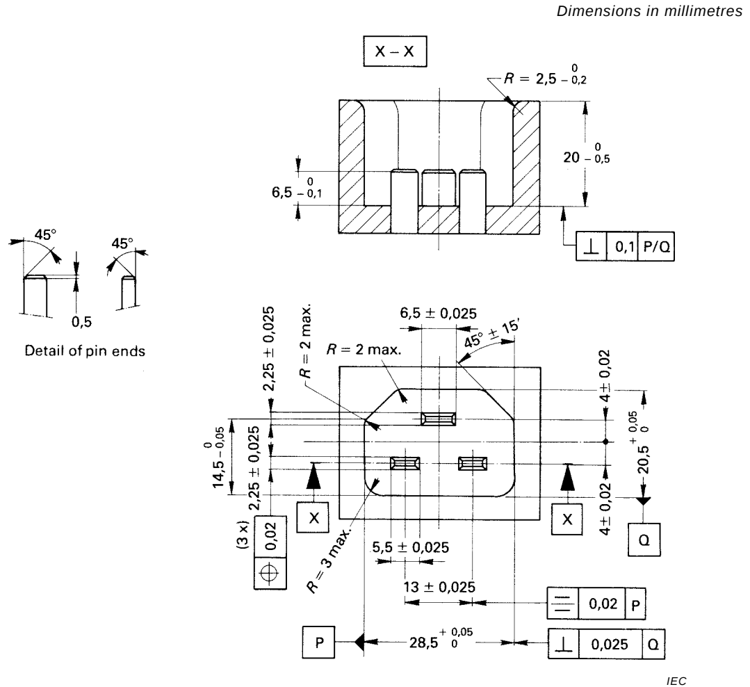
Figure 21 – "GO" gauge for connectors to standard sheet C21
