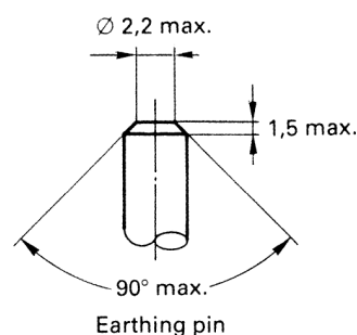
Earthing pin
