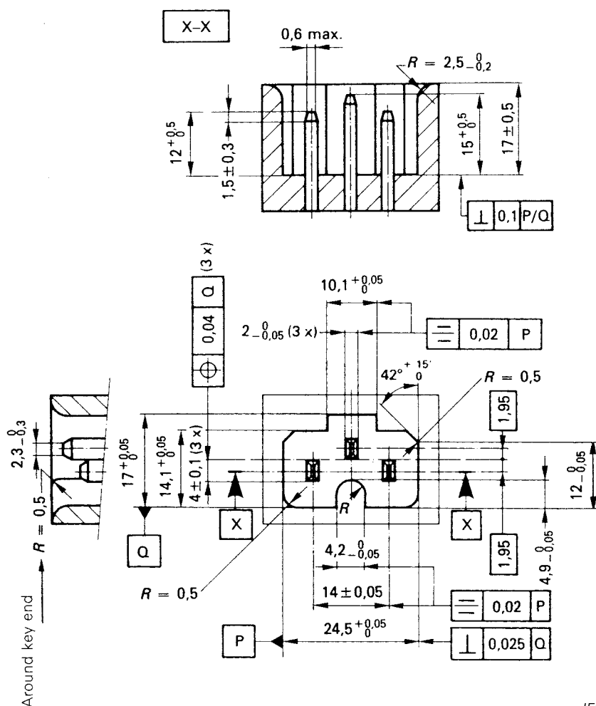
Figure 24 – "NOT-GO" gauge for connectors to standard sheets C13, C15 and C17
