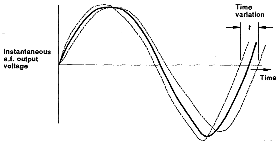
Figure 6 - Measurement of peak frequency deviation due to residual f.m., vibration or shock (see 2.15.1)
