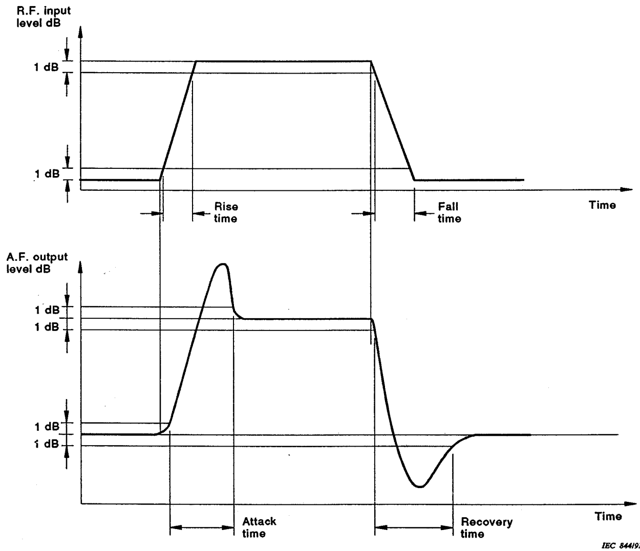
Figure 4 - Results of the measurement of a.g.c. response time characteristics (see 2.5.1 and 2.5.2)
