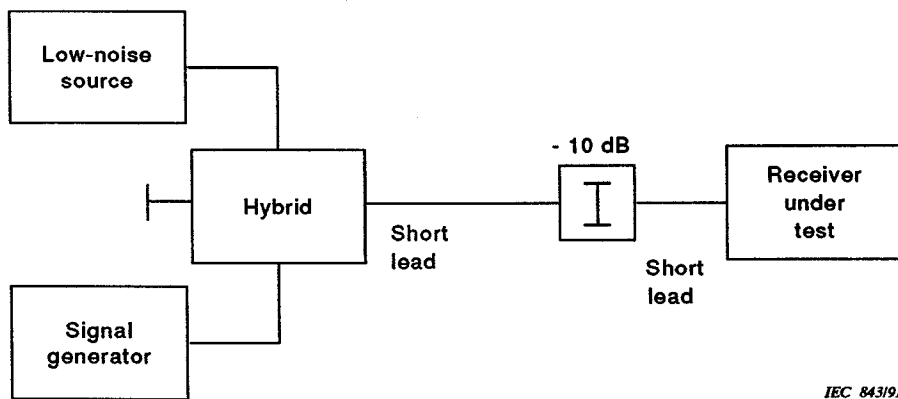
Figure 3 - Measuring arrangement for third-order intercept level (see 2.8.1)
