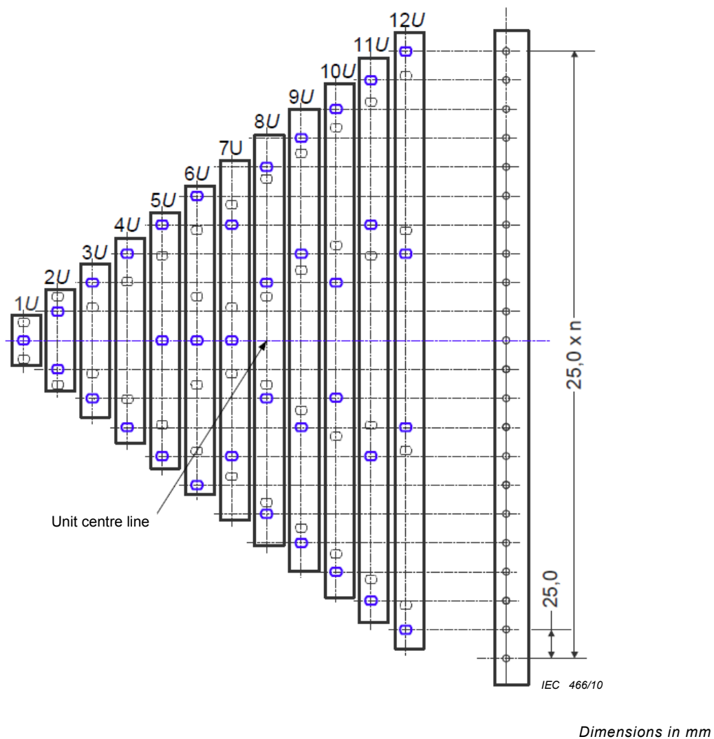
Figure 4 – Mounting hole arrangements on the flanges, mounting layout referred to the unit centre lines of the 19 in subracks or chassis
