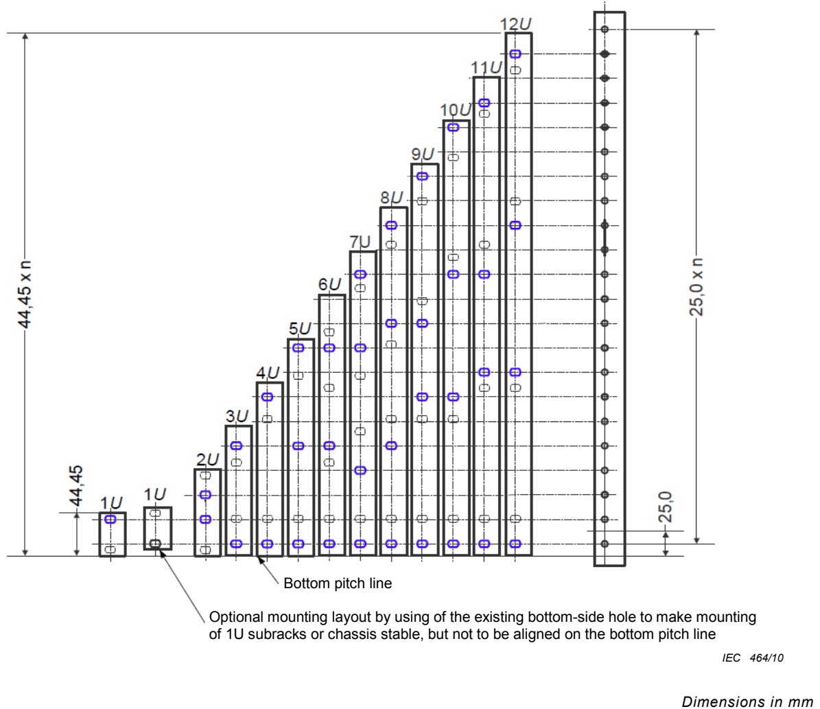
Figure 2 – Mounting hole arrangements on the flanges, mounting layout referred to the bottom pitch lines of the 19 in subracks or chassis
