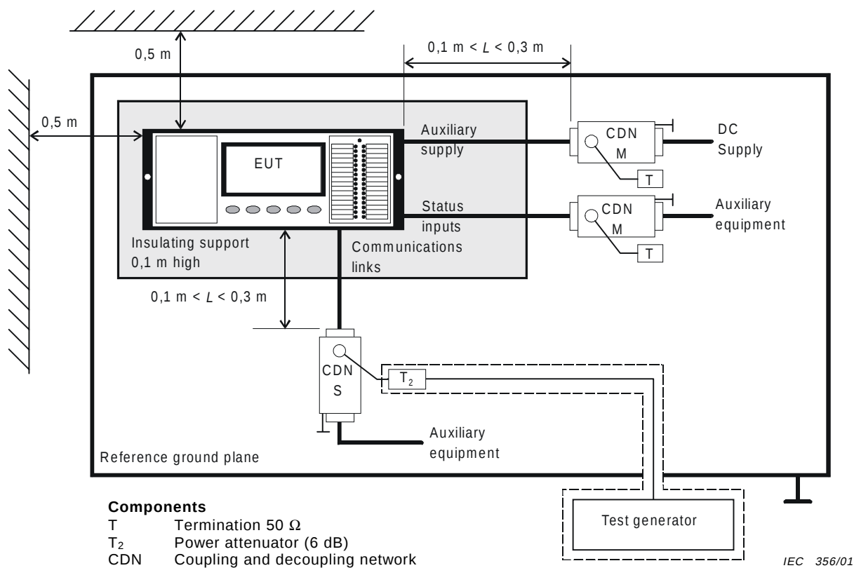
Figure 2 – Example of a test set-up using CDNs for single equipment
