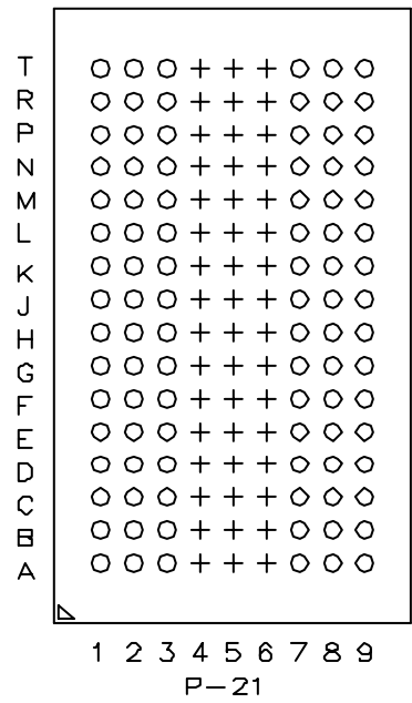
FIGURE 3 : SOLDER BALL PATTERNS
