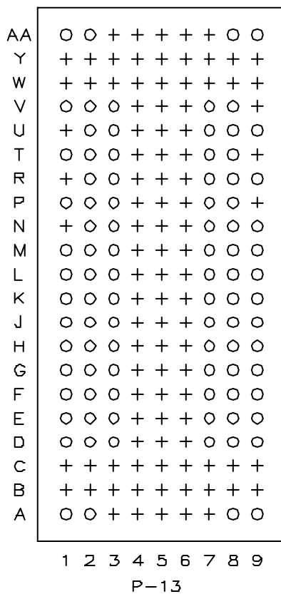
FIGURE 3 : SOLDER BALL PATTERNS (CONT'D)
