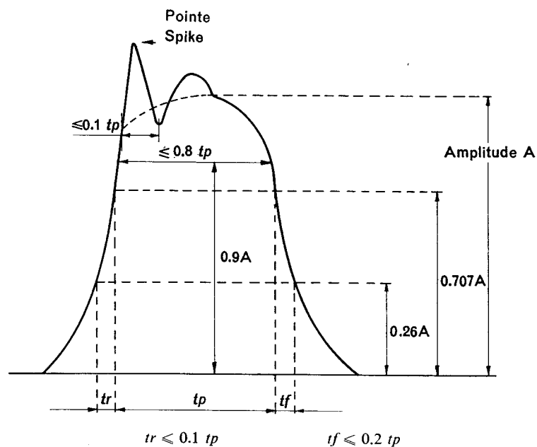
FIG. 5. — Forme d'impulsion type. Typical pulse shape.
