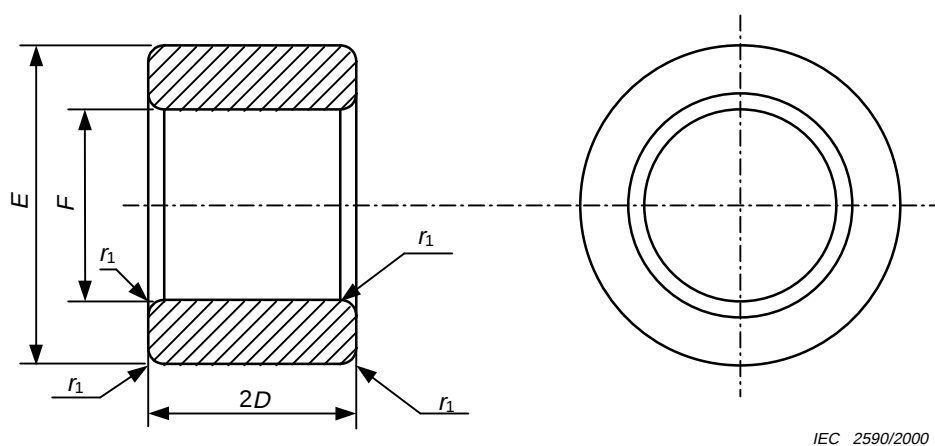
Figure C.1 – Dimensions of gauge A
