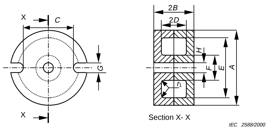
Figure 2 – Principal dimensions of pot-cores with slots
