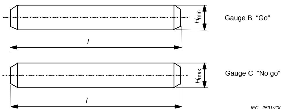
Figure C.2 – Dimensions of gauges B and C
