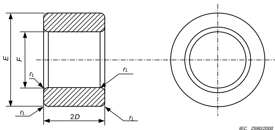
Figure C.1 – Dimensions du calibre A
