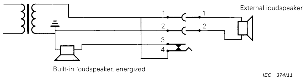
Figure C.1 – Free connector 60130-9 IEC-05 inserted in position A
