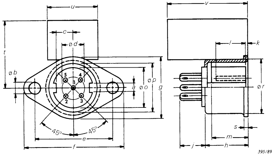
Figure 16 – Embase 60130-9 IEC-15a
