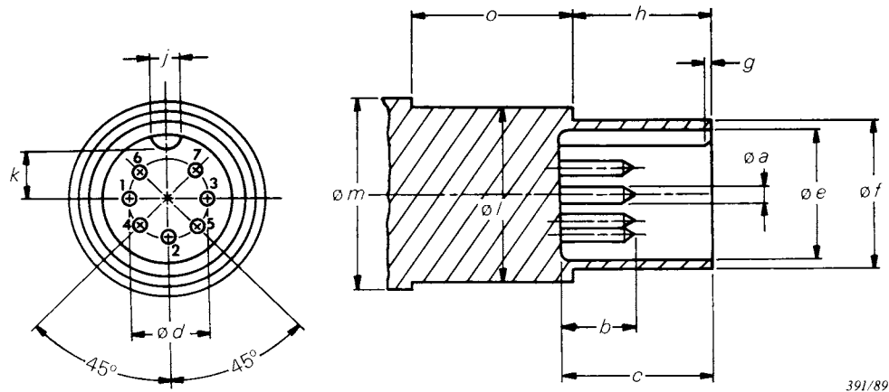
Figure 12 – Fiche 60130-9 IEC-12
