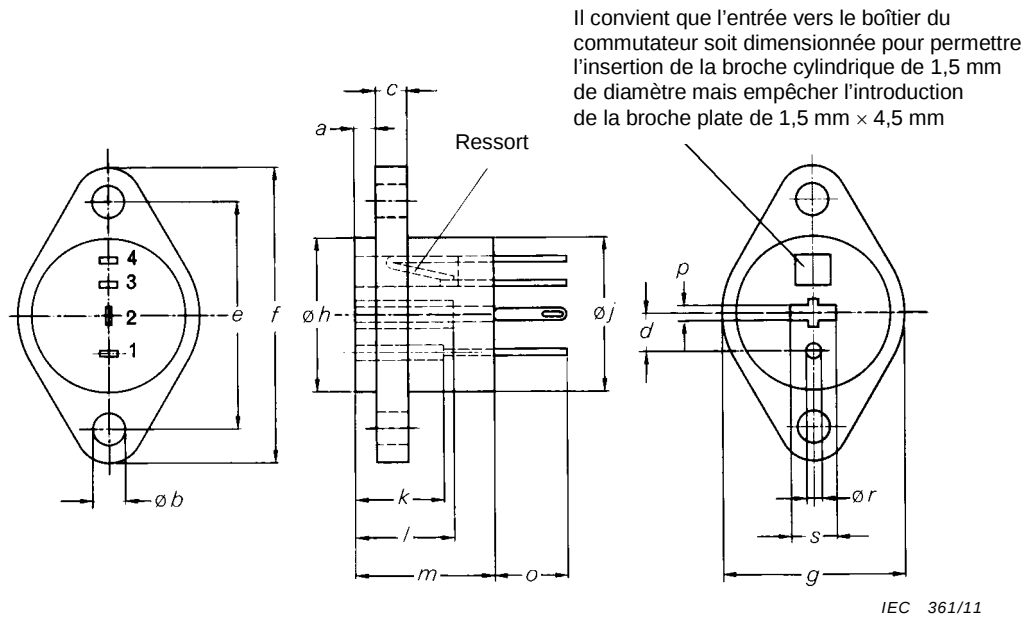
Figure 8 – Embase 60130-9 IEC-08
