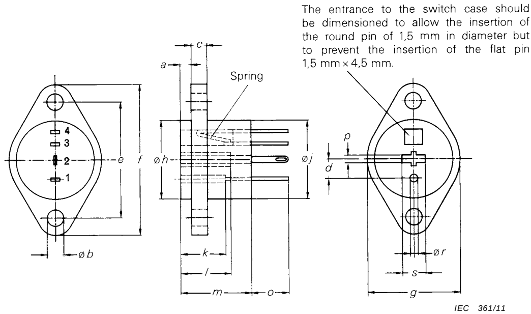
Figure 8 – Fixed connector 60130-9 IEC-08
