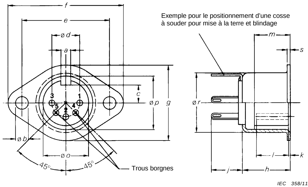
Figure 2 – Embase 60130-9 IEC-02
