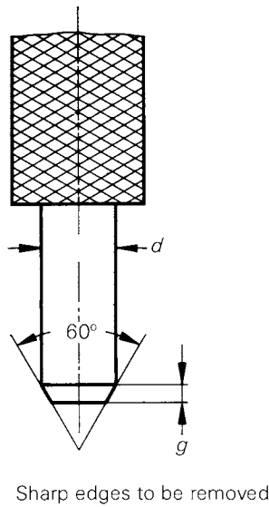
Figure 32 – Gauge for connector types 60130-9 IEC-07, 08 and 09
