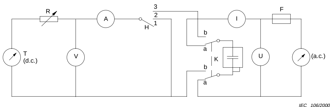
Figure 1 – Circuit for performing the destruction test
