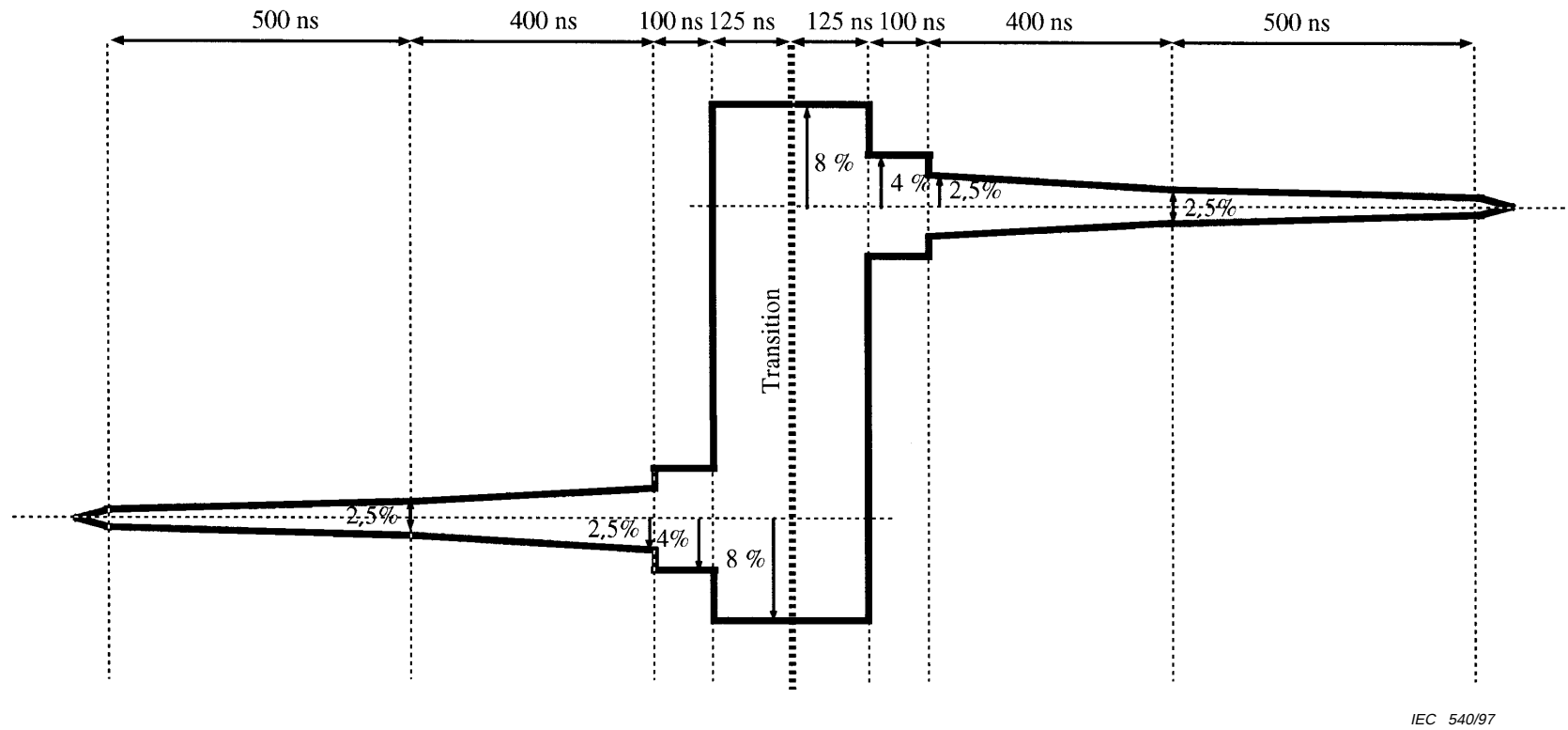
Figure 10 – A mask for the response to a shaped step
