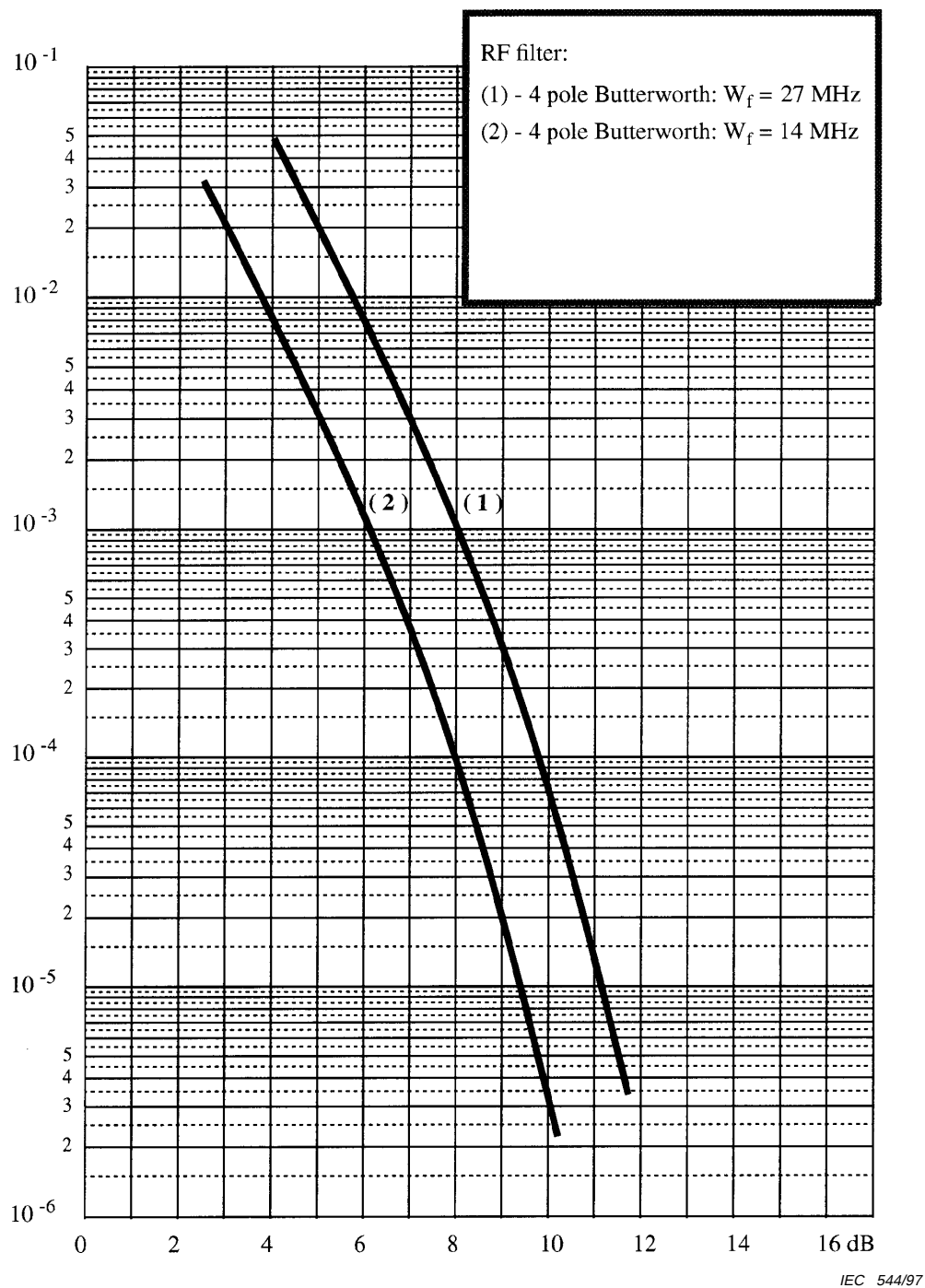
Figure A.2 – Theoretical bit error ratio as a function of C/N (noise measurement bandwidth W = 27 MHz)
