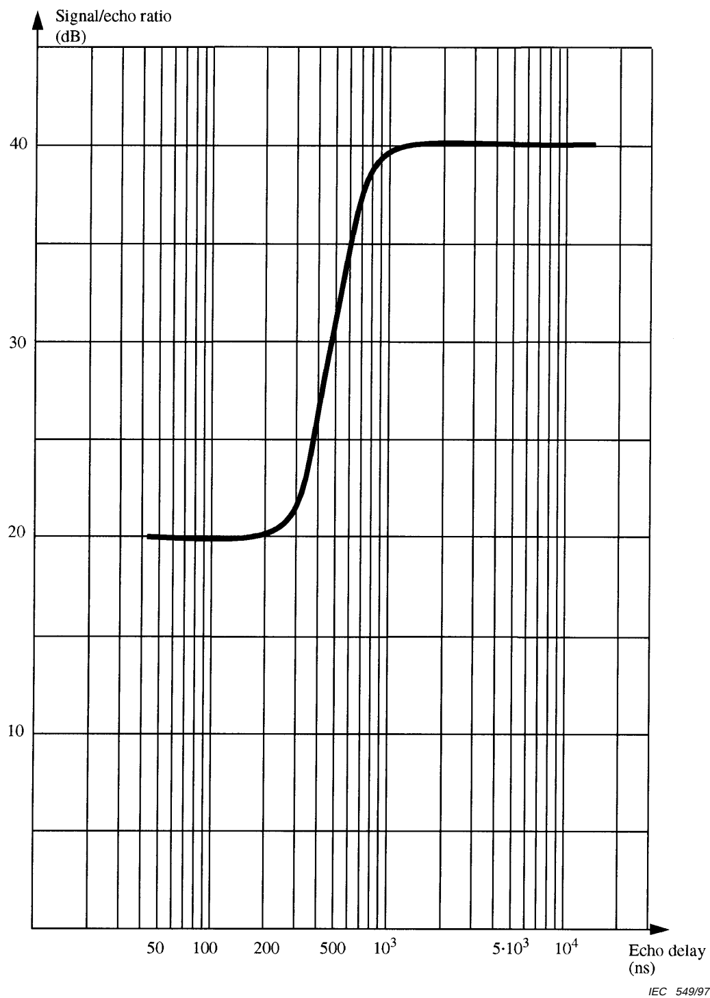
Figure B.2 – Example of acceptable signal-to-echo ratio in D2-MAC/packet AM-VSB
