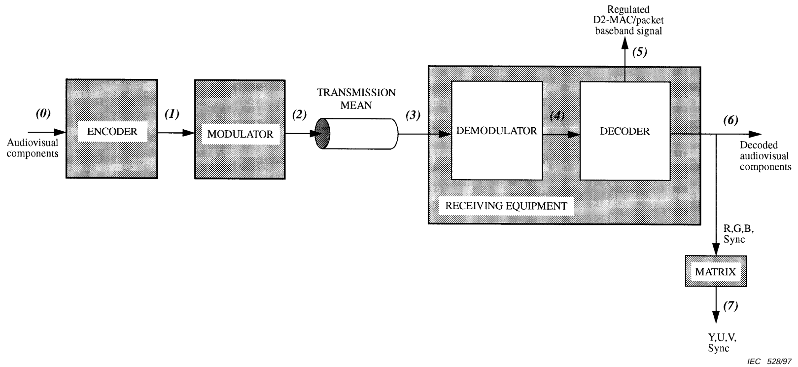
Figure 1 – Hypothetical reference chain notional block diagram
