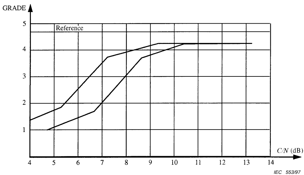
Figure B.5 – Result of measurement on picture signal quality as a function of C/N in 27 MHz bandwidth
