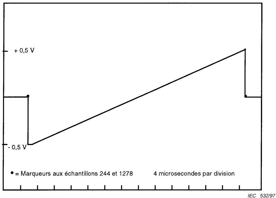
Figure 4a – Trames paires
