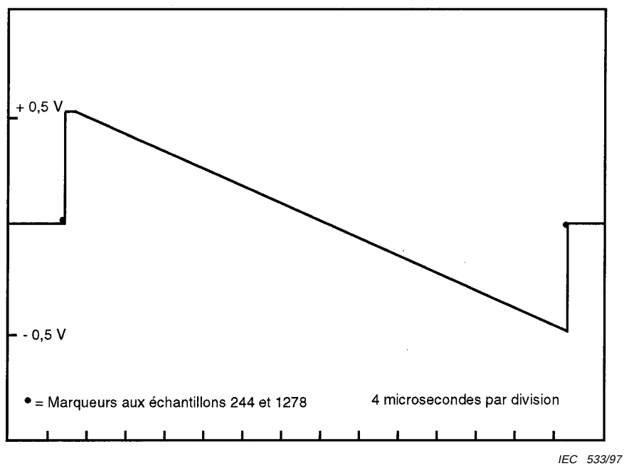
Figure 4b – Trames impaires
