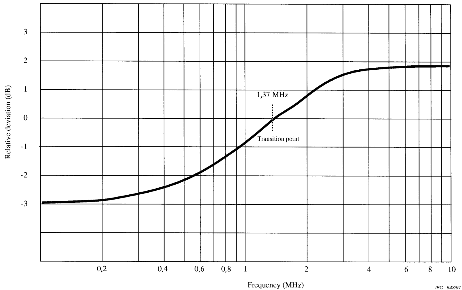
Figure A.1 – Pre-emphasis for D2-MAC/packet
