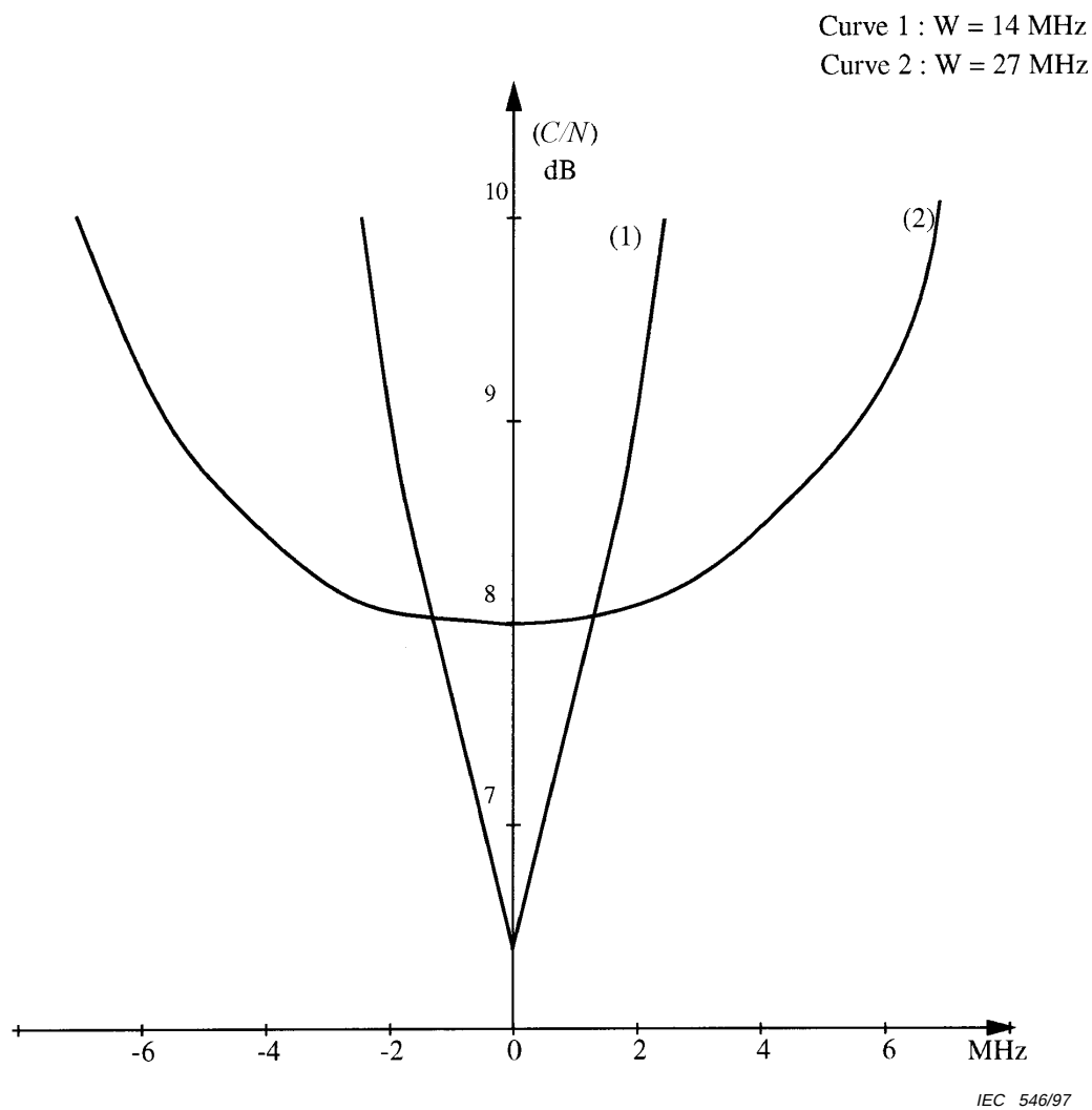
Figure A.4 – Example of equivalent degradation for a carrier frequency shift at the 10^{-3} bit error ratio
