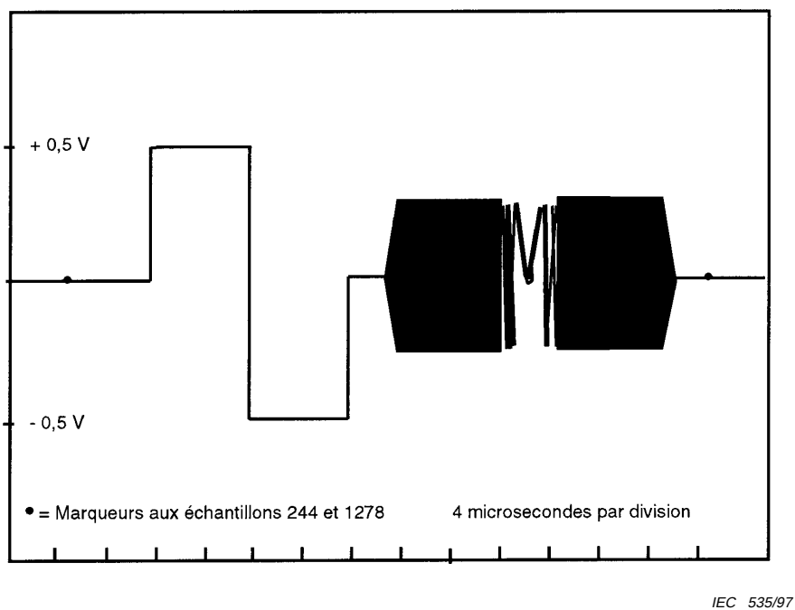
Figure 5b – Trames impaires
