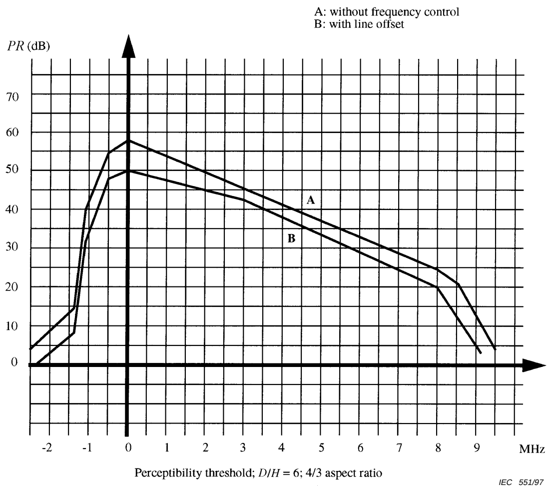
Figure B.4 – Example of protection ratio against interference in AM-VSB
