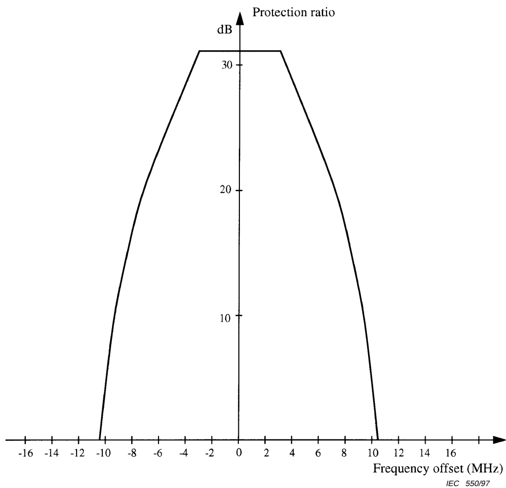
Figure B.3 – Example of protection ratio against interference in FM
