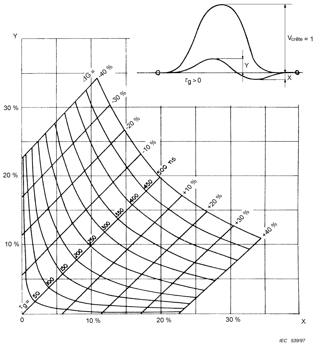
Figure 9 – Abaque de Rosman
