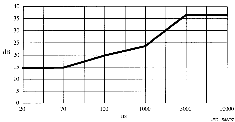
Figure B.1 – Example of acceptable signal-to-echo ratio in D2-MAC/packet in FM
