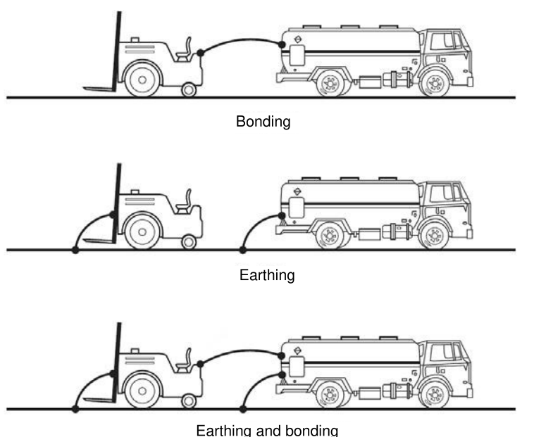
Figure 4 – Difference between earthing and bonding
