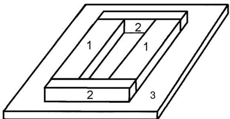
Figure G.2 – Measuring cell for powder resistivity
