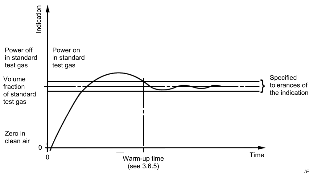
Figure 2 – Warm-up time in standard test gas (typical)
