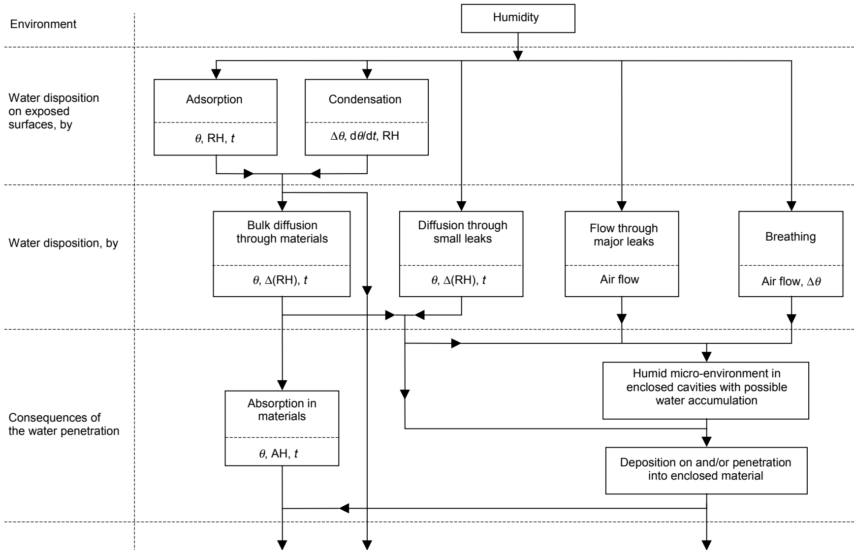
Figure A.1 – Physical processes involved in humidity testing
