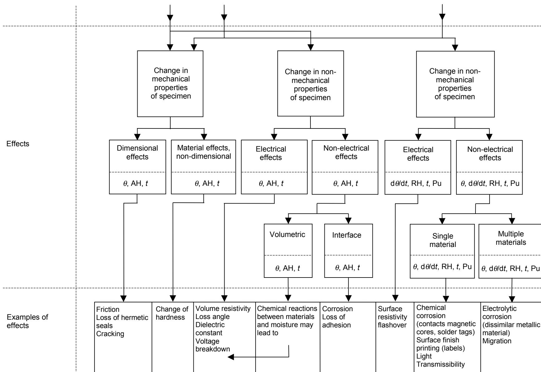
Figure A.1 – Physical processes involved in humidity testing (continued)
