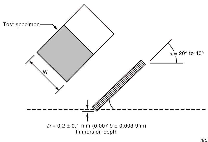
Figure 6 – Printed board immersion
