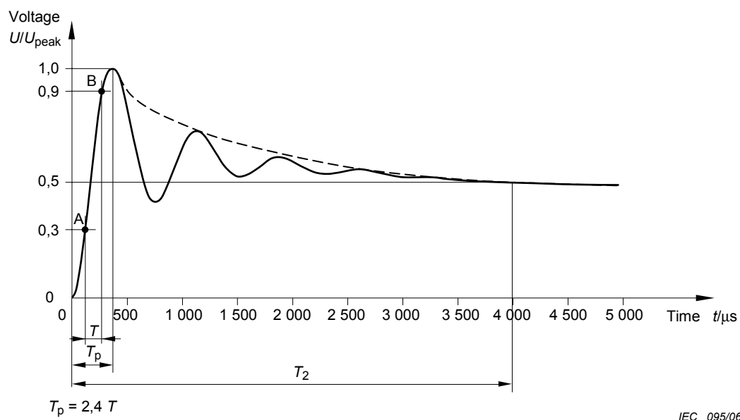
b) T_p/T_2 = 400/4\,000\ \mu\text{s}, 1\ \text{kHz}
