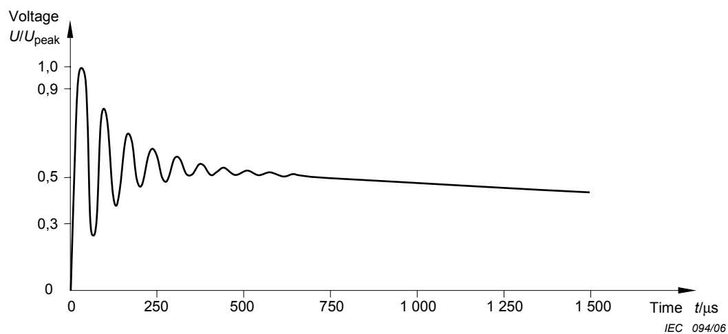
a) T_p/T_2 = 20/1\,000\ \mu\text{s}, 15\ \text{kHz}
