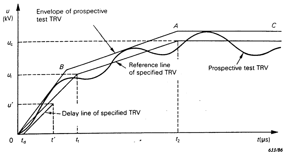
23. — Example of prospective test TRV with four-parameter envelope which satisfies the conditions to be met during type test: case of specified TRV with four-parameter reference line.
