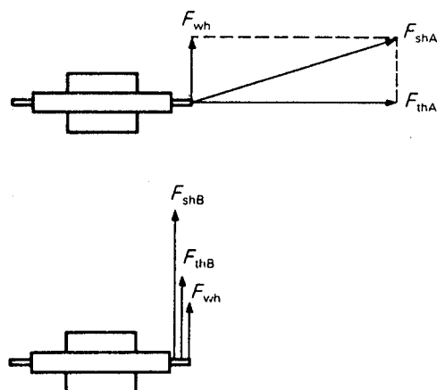
Horizontal forces
