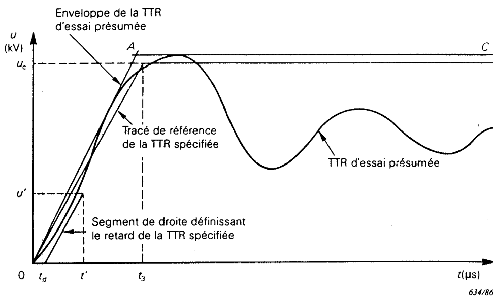
24. — Example of prospective test TRV with two-parameter envelope which satisfies the conditions to be met during type test: case of specified TRV with two-parameter reference line.
