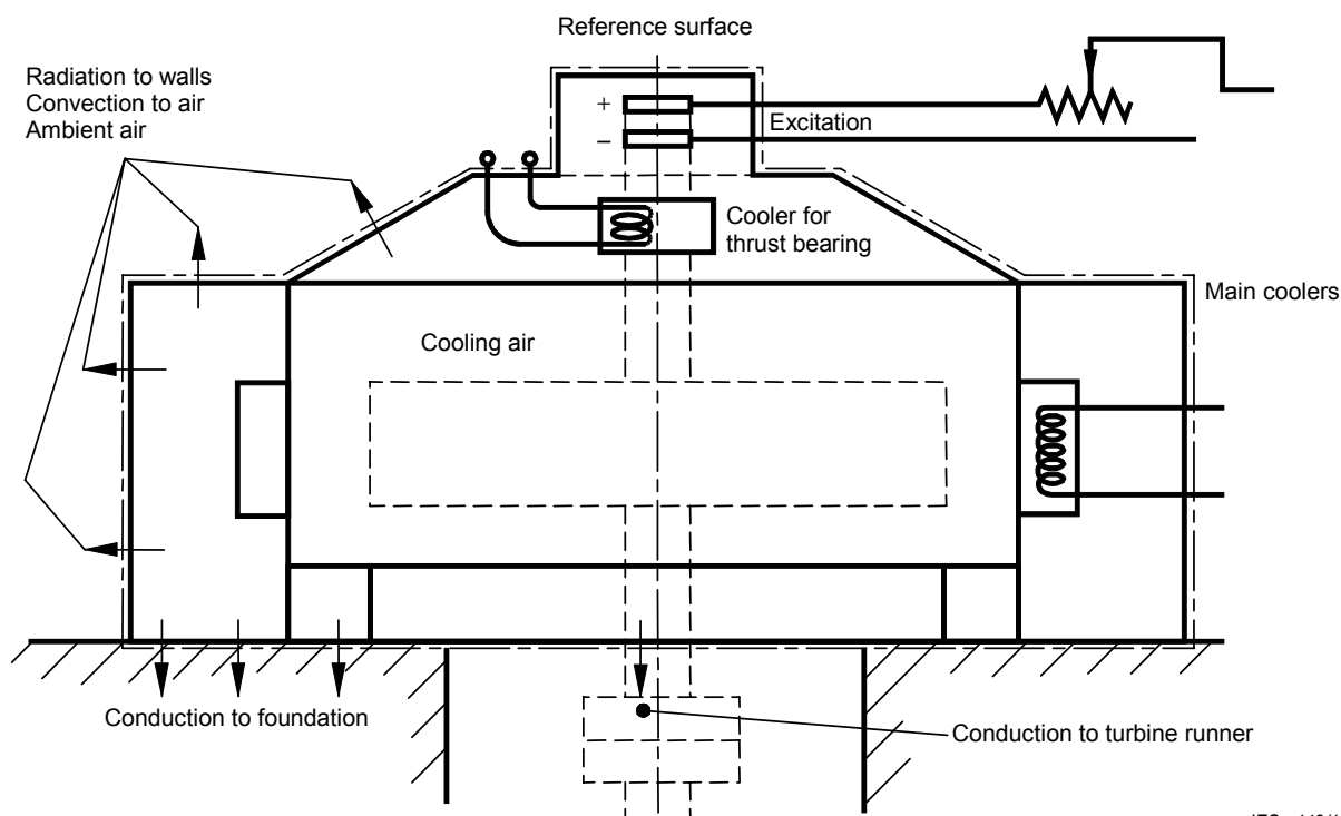
Figure 2 – Reference surface
