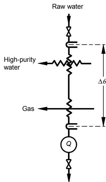
Figure 4 – Series connected coolers, two coolants
