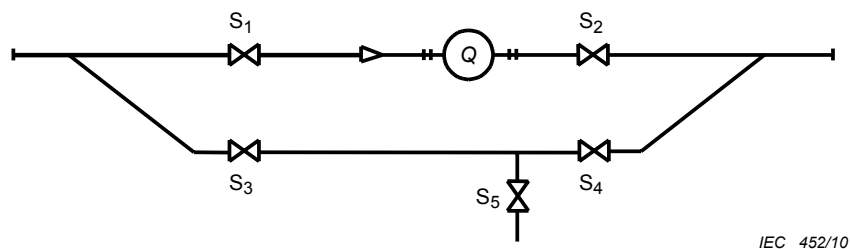
Figure 5 – Bypass piping
