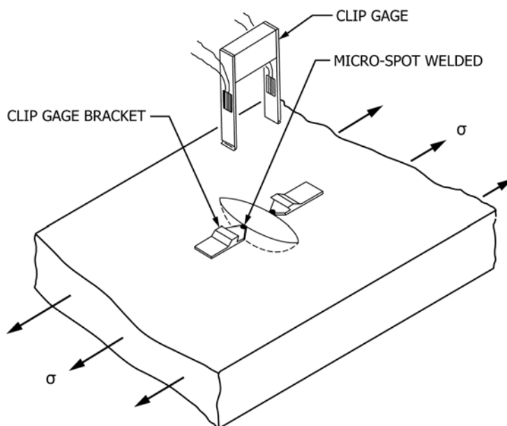
FIG. X2.1 Typical Experimental Setup for CMOD Measurement
