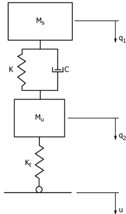
FIG. 1 Quarter-Truck Model
