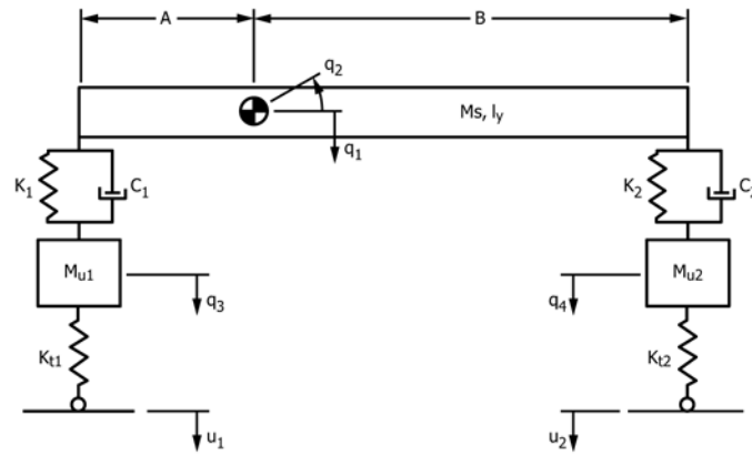
FIG. 2 Half-Single Unit Truck Model
