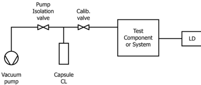
FIG. 4 Calibration Setups
