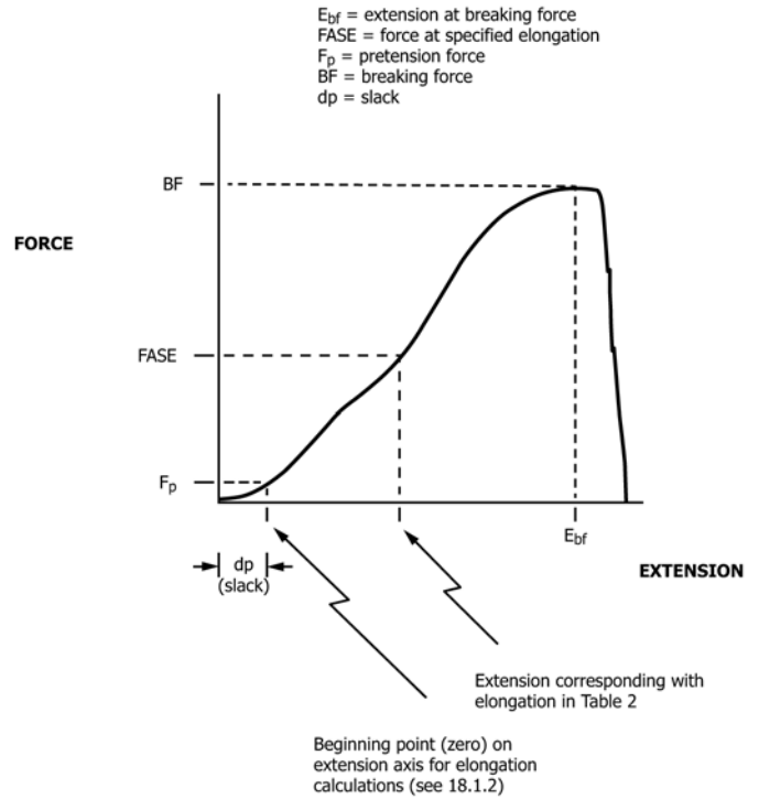
FIG. 1 Force-Extension Curve
