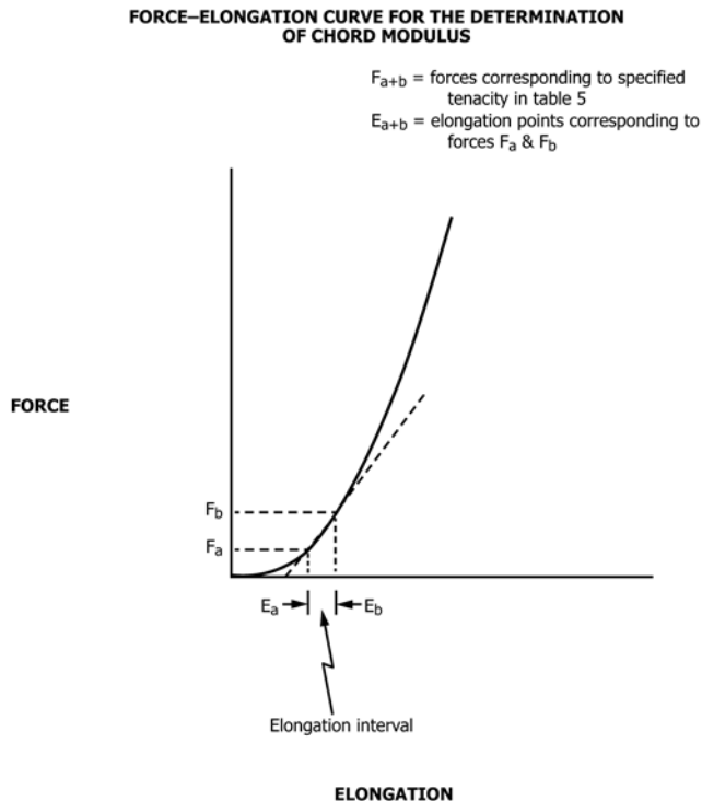
FIG. 3 Force-Elongation Curve for the Determination of Chord Modulus
