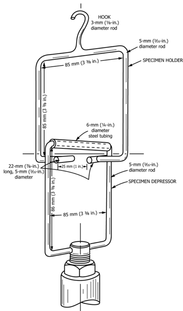
FIG. 4 Apparatus for Stiffness of Fabric Testing
