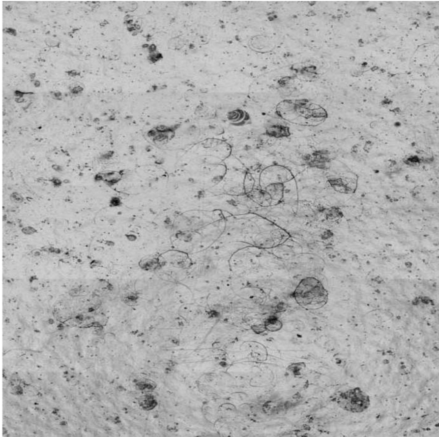
FIG. X1.4 Digital Image of Acid Etch Produced by the Exposure Described in This Standard (actual size 4 × 6 in.). Black Basecoat/Clearcoat System on Cold Rolled Steel
