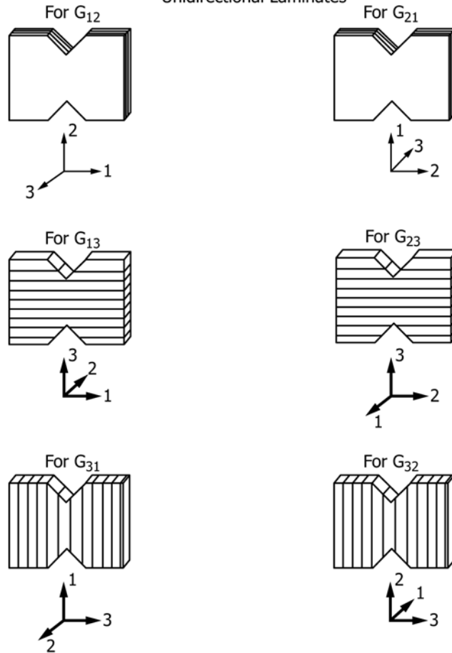
FIG. 9 Orientation of Material Planes
