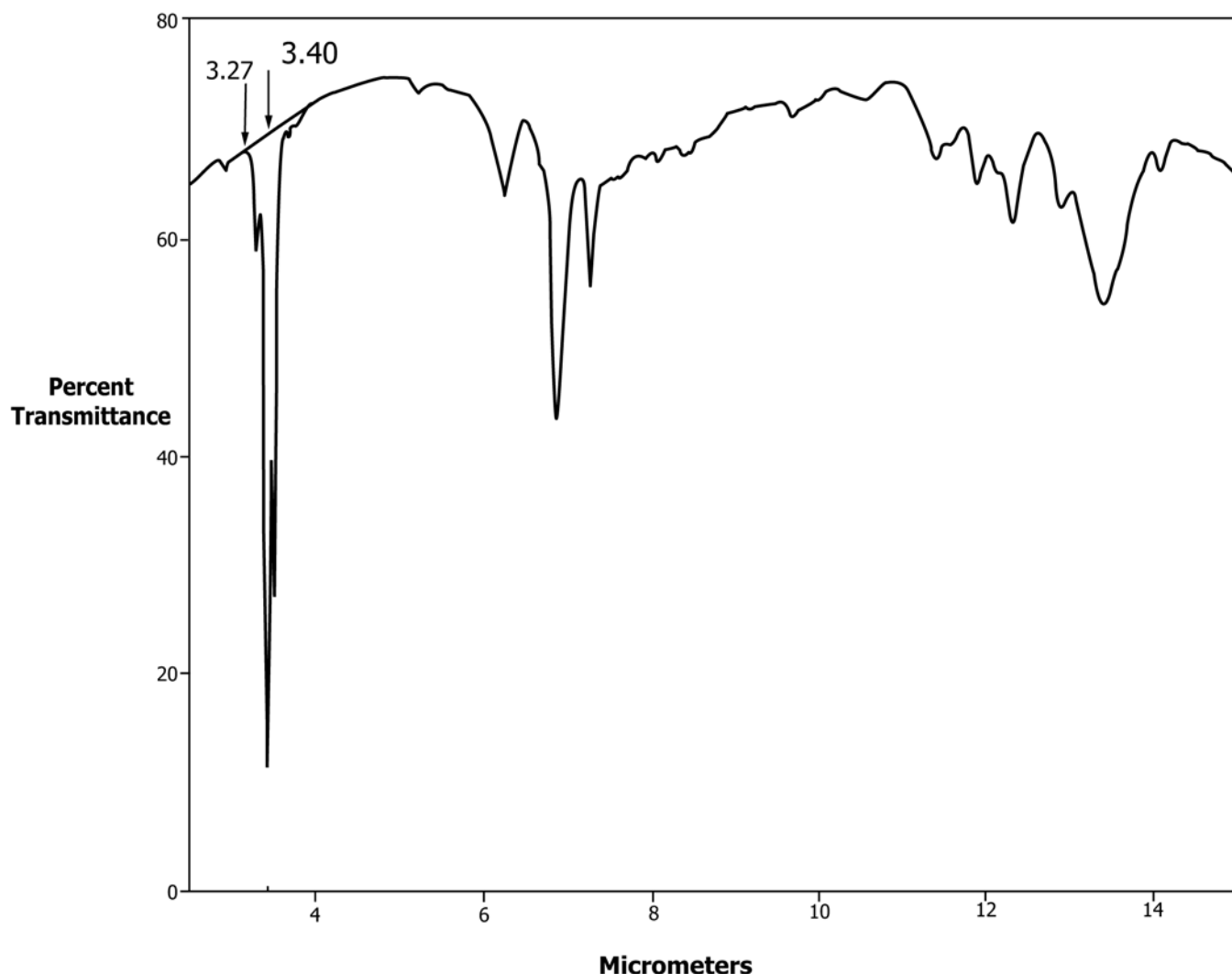
FIG. X2.2 Transmittance Graph
