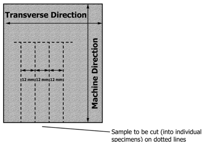
FIG. 2 Typical Sample of a Pressure Sensitive Article (Schematic for Sample Preparation)
