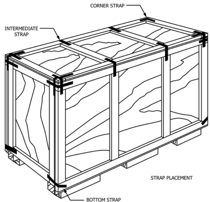
FIG. 8 Strap Placement
