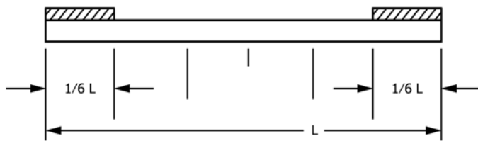
LOAD CONDITION A LOAD BEARING POINTS ON OUTER ONE-SIXTHS OF SKID LENGTH
