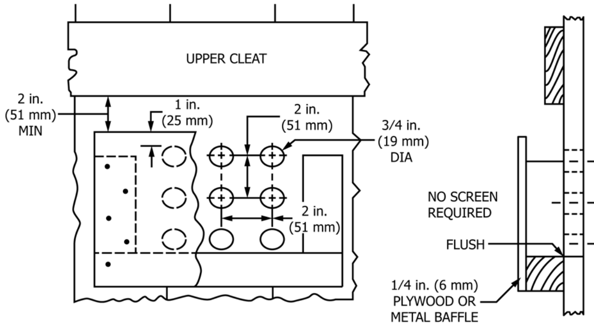
VENTILATION HOLES
