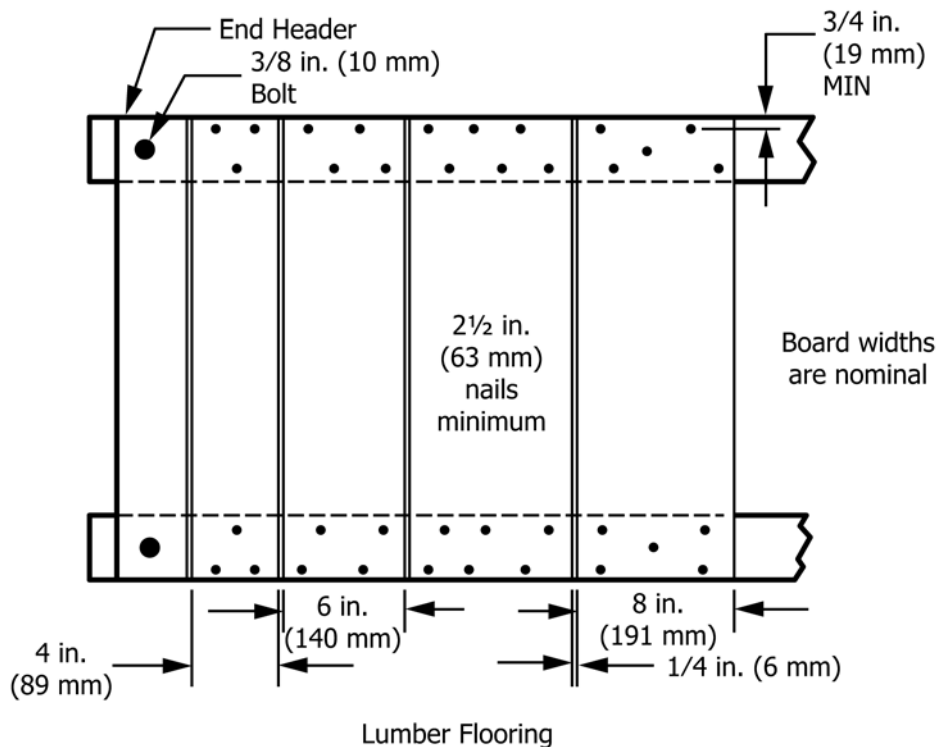
FIG. 5 Nailing Patterns For Base
