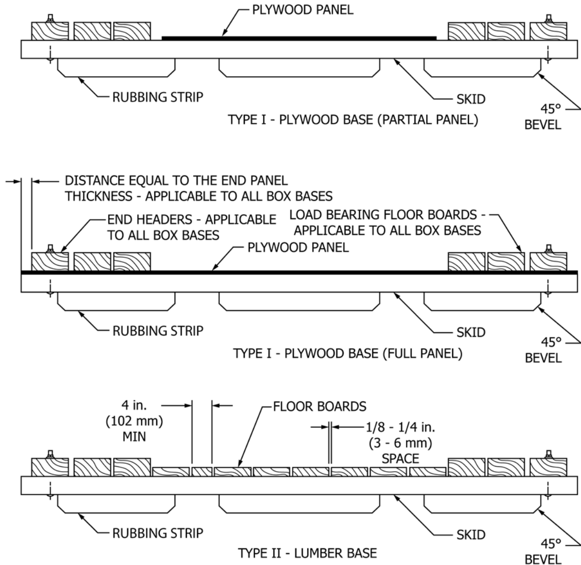
FIG. 1 Base Types
