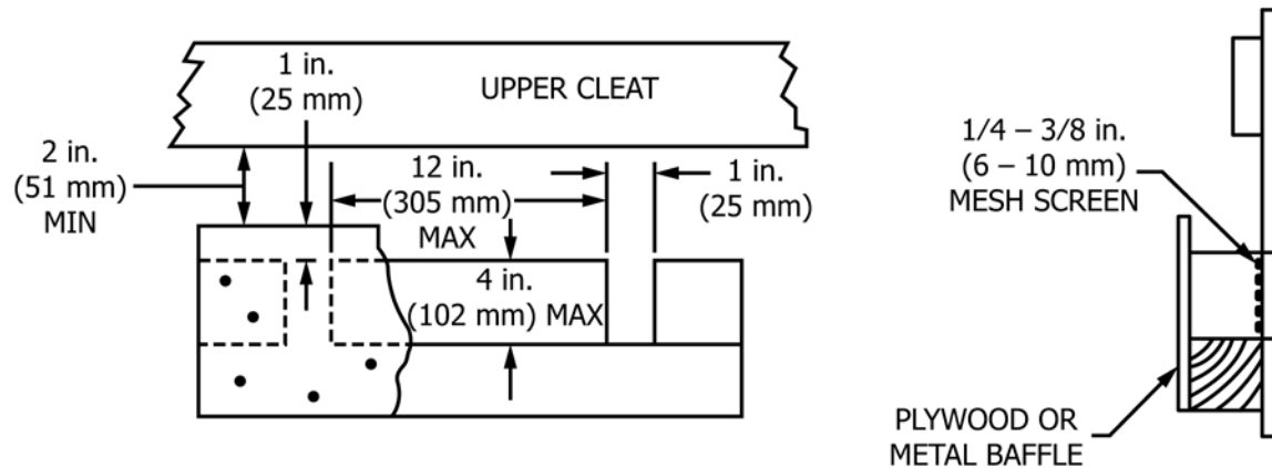
VENTILATION SLOTS
