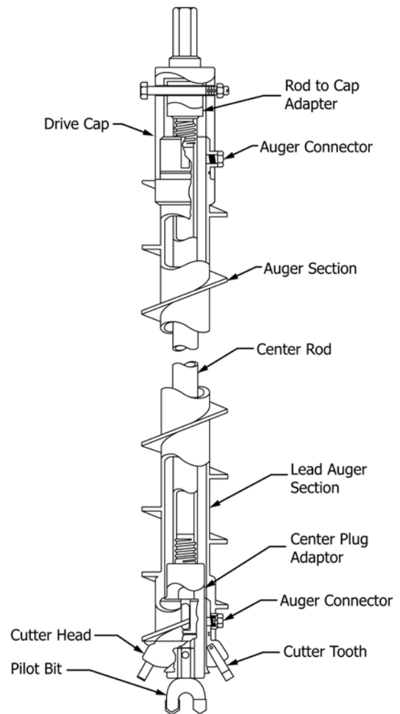
FIG. 1 Rod-Type Auger System With Pilot Bit
