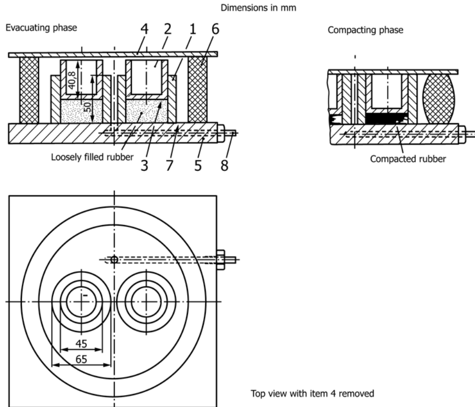
FIG. A1.1 Vacuum Compaction Apparatus
