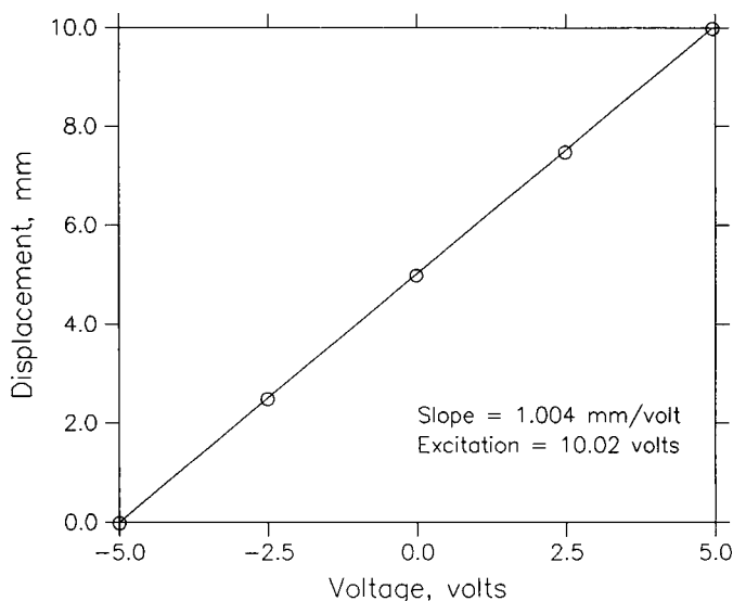
FIG. 1 Displacement Transducer Calibration
