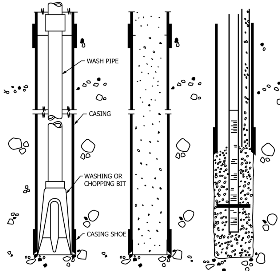
FIG. 2 Basic Three-Step Procedure for Installation of Instrumentation Devices Using Casing Advancement Methods
