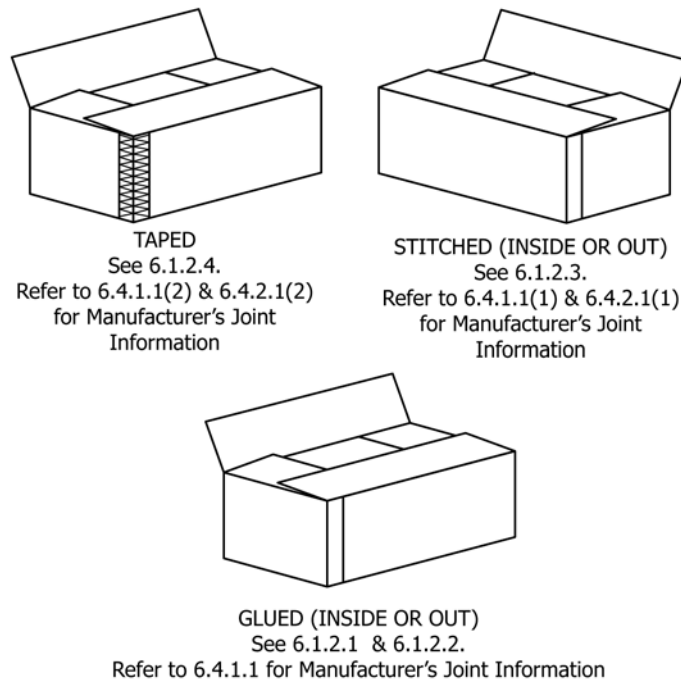
FIG. 3 Box, Fiberboard; Details of Manufacturer's Joint Types
