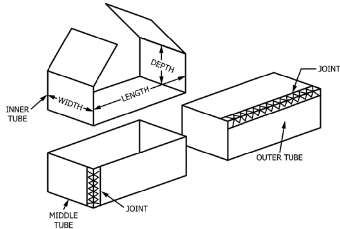
FIG. 22 Box, Fiberboard; TS—Triple Slide Box
