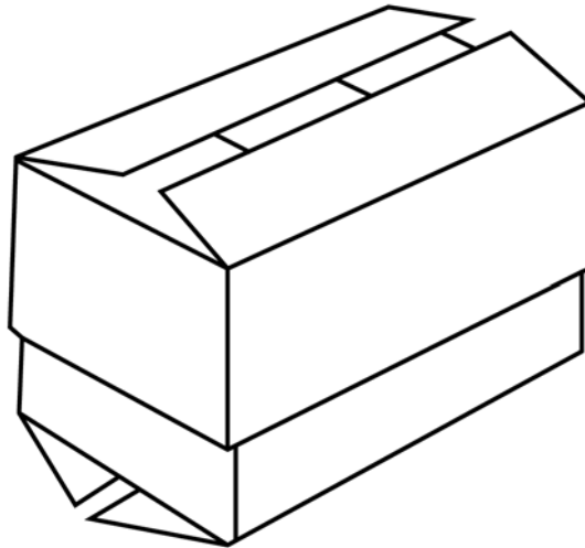
FIG. 17 Box, Fiberboard; FTHS—Two Piece Full Telescope Half Slotted Box (0320)
