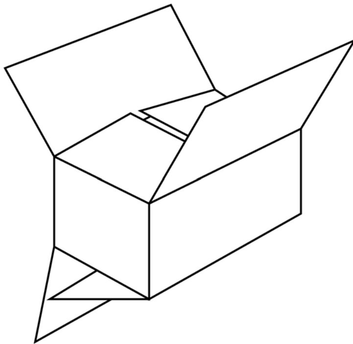
FIG. 11 Box, Fiberboard; SFF—Special Full Flap Slotted Box (0206)
