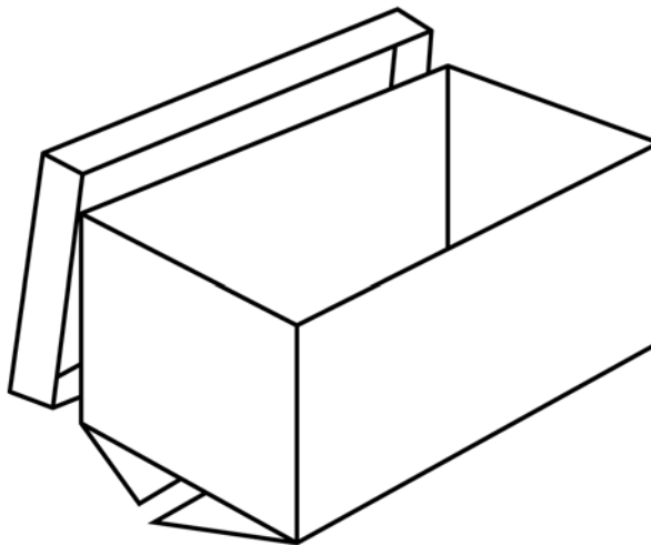
FIG. 13 Box, Fiberboard; HSCC—Half Slotted Box with Cover (0200)
