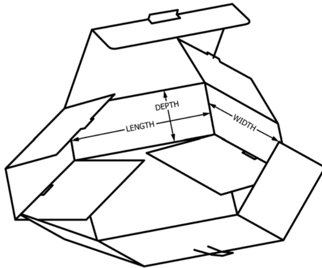
FIG. 21 Folder, Fiberboard; TSC—Tongue and Slot Closure
