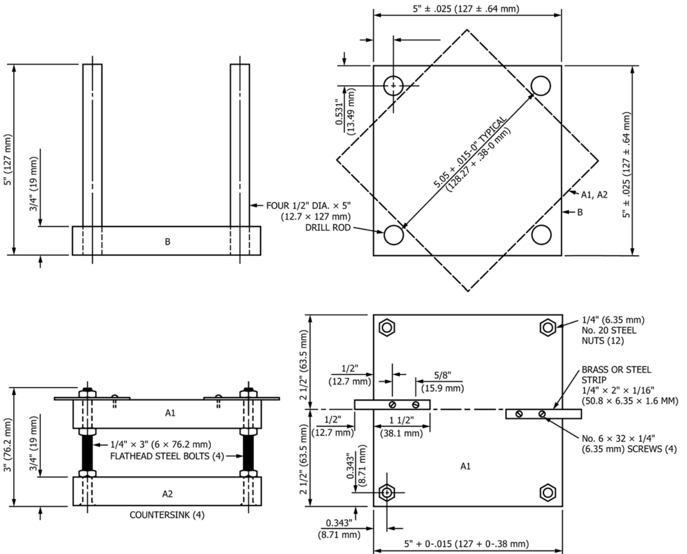
FIG. 2 Plastometer Details
