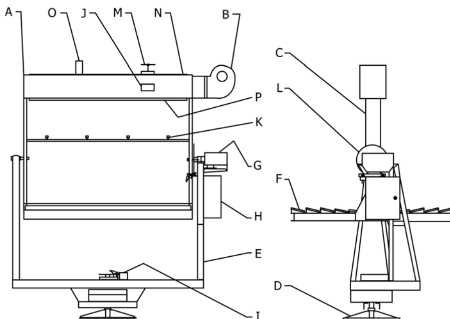
FIG. 3 Fresnel Reflector Diagram (from Practice G90)
