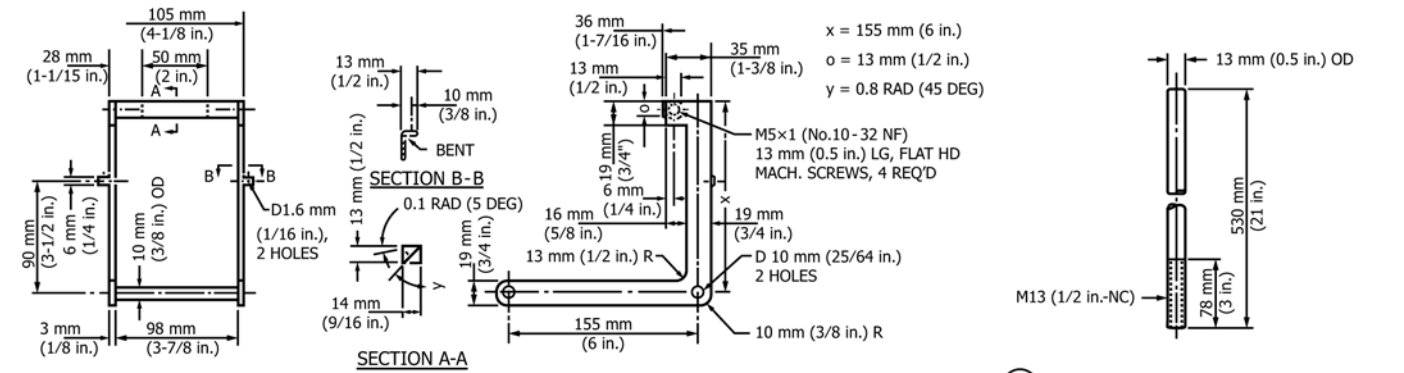
2 YOKE COLUMN, STEEL ROD, TWO REQ'D
