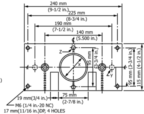
FIG. 14 Holding and Lowering Device (Additional Details)
