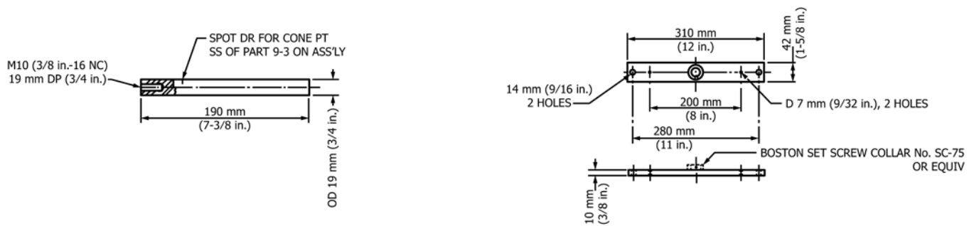
3 PISTON ROD-STEEL, ONE REQ'D
