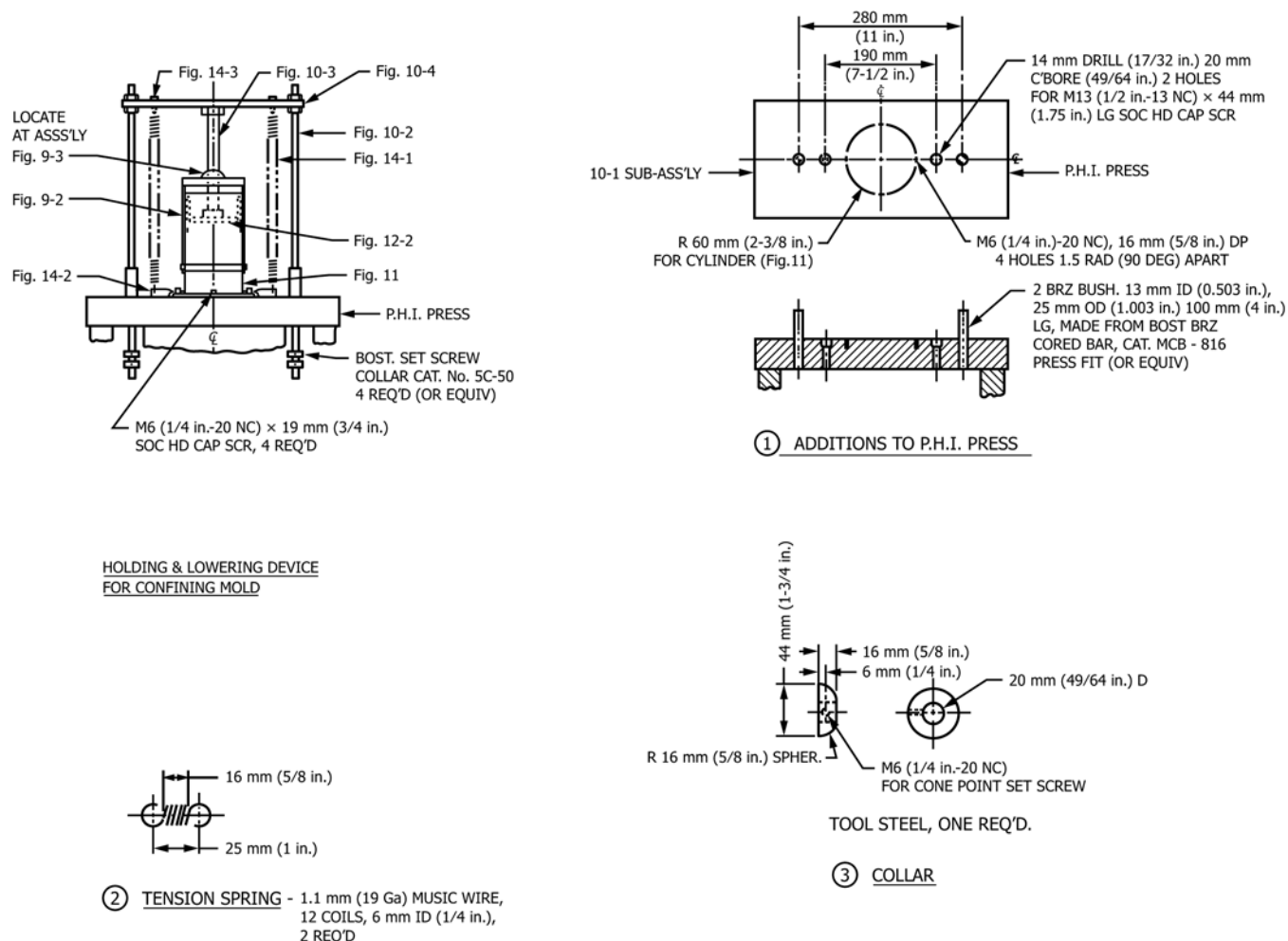
FIG. 9 Holding and Lowering Device Assembly and Details for Parts 2 and 3 of the Assembly
