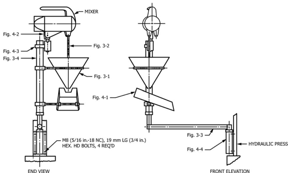
FIG. 1 Wet-Mixer Assembly
