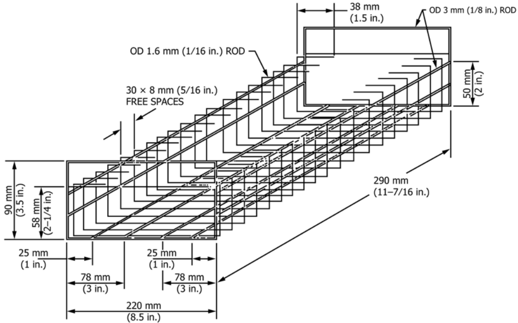
FIG. 23 Specimen Basket
