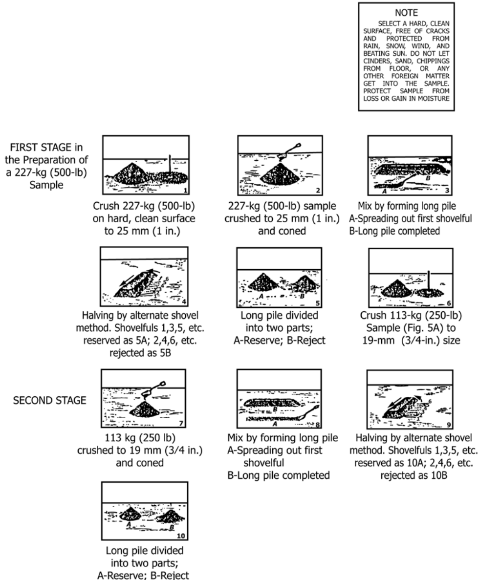
FIG. 2 Standard Hand Method of Crushing and Reducing the Gross Sample Quantity of Coke
