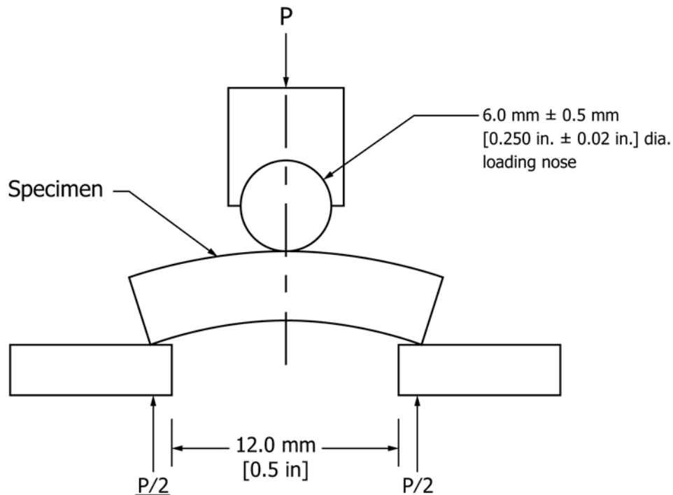
FIG. 5 Horizontal Shear Load Diagram (Curved Beam)
