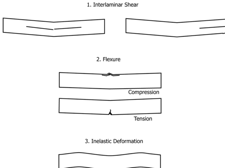
FIG. 7 Typical Failure Modes in the Short Beam Test
