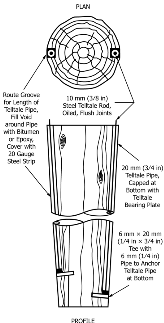
Note: Install Telltale Rods After Driving FIG. 10 Possible Installation of Telltales for Timber Piles
