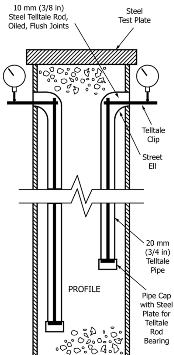
Note: Install Telltale Pipes, Install Telltale Rods, and Fill Pipe with Concrete After Driving FIG. 9 Possible Installation of Telltales for Pipe Piles
