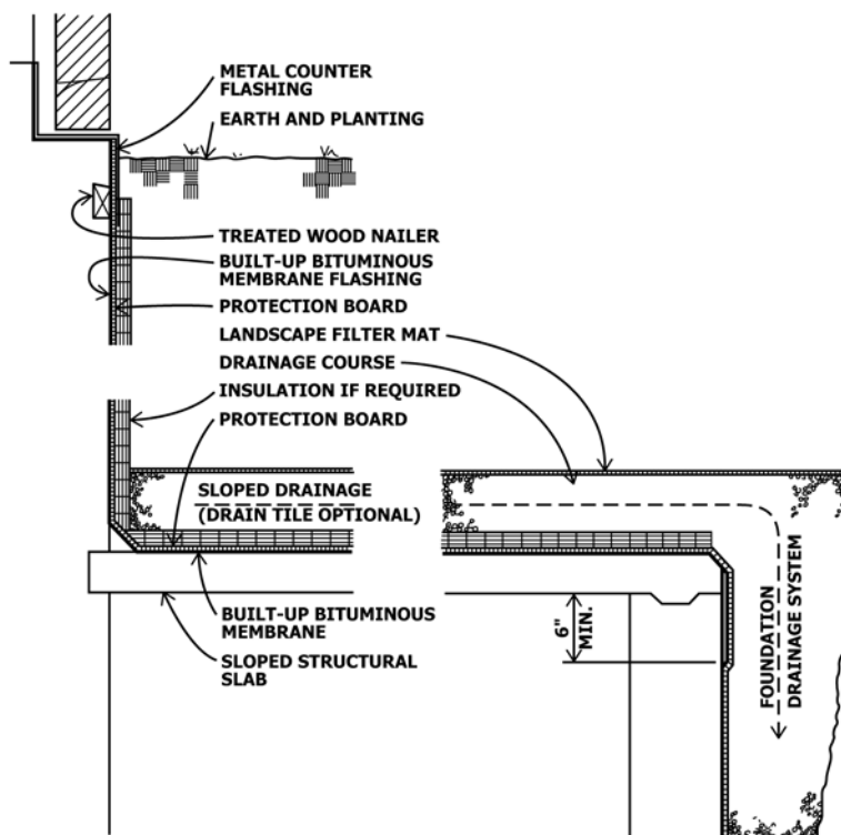
FIG. 12 Earth Fill and Planted Areas (see 15.1)
